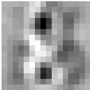
weight vector
