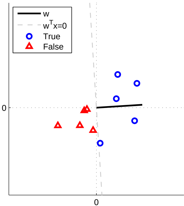
Step 4, 0 Misclassified
