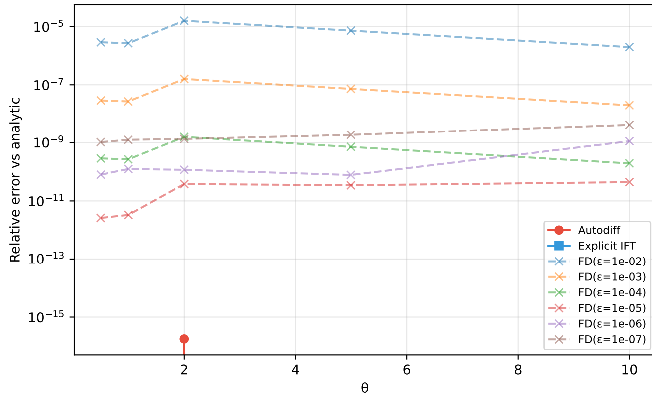
Problem 1: Toy Implicit Root
