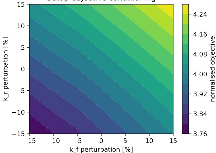
Setup-objective conditioning
