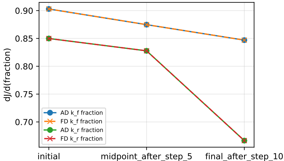
AD versus FD setup gradients
