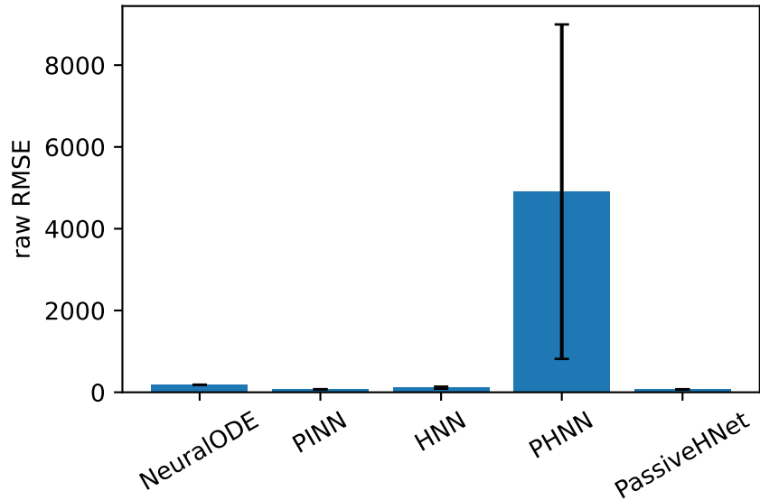
200-step rollout RMSE
