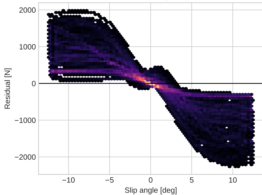
Error versus slip angle
