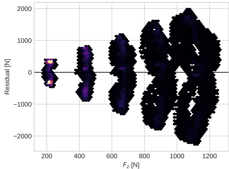
Error versus normal load
