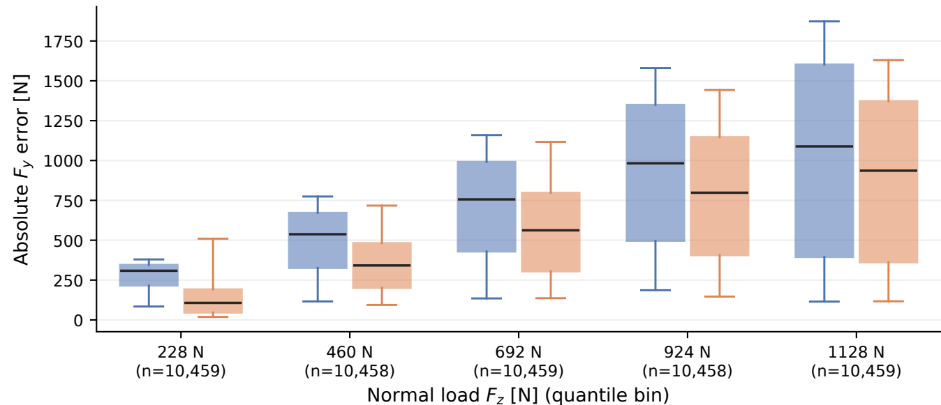
Held-out Run 6: error distribution by normal load
