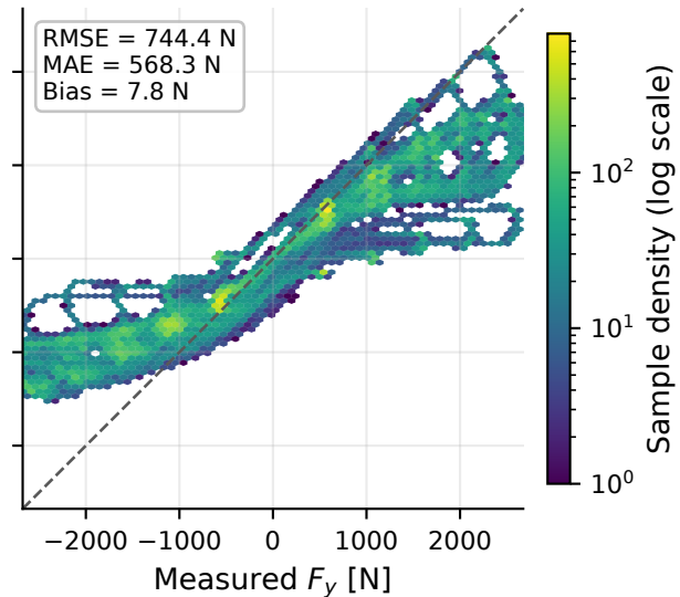
Pacejka + residual NN
