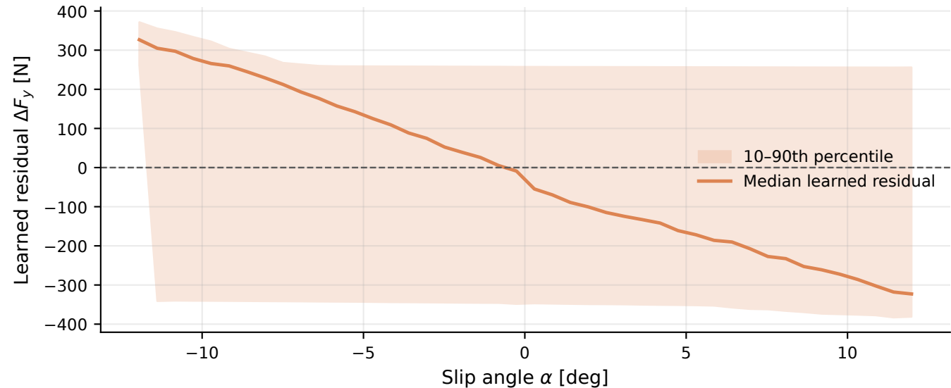
Learned residual correction on held-out TTC Run 6
