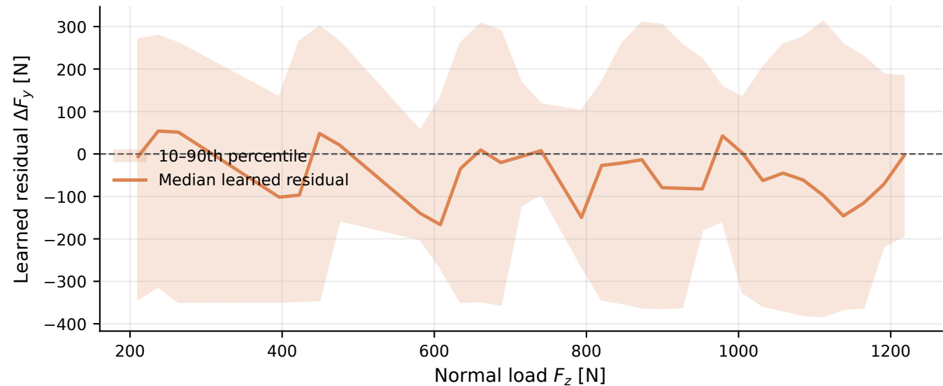
Learned residual correction vs. normal load, held-out Run 6
