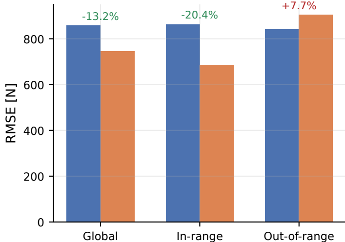
Lateral-force RMSE
