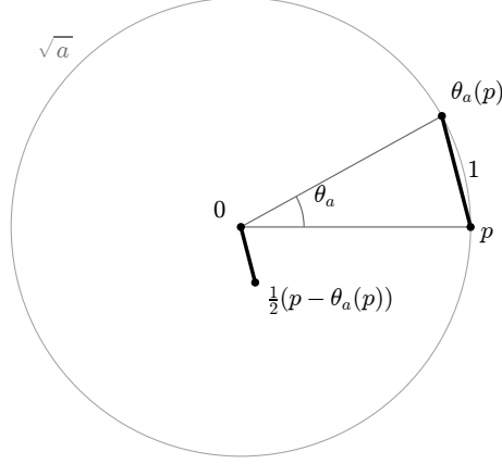
FIGURE 2. The spindle at squared radius a . Two shell points at distance \sqrt{a} are carried onto each other by \theta_a and land at distance exactly 1, which is what the rotation is for. Half that displacement has length \frac{1}{2} always, since |1 - \theta_a| = 1/\sqrt{a} ; whether it lies in the lattice is the whole content of Theorem 1. Drawn for a = 4 , \cos \theta_4 = 7/8 .
