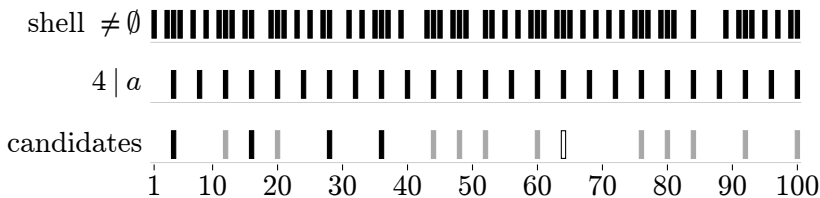
FIGURE 2. Theorem 1 as a sieve, over the integer spindles a \leq 100 . Top: the 59 positive squared radii at which R has points, decided by the form (3) rather than by a ball, and in closed form by Theorem 18. Middle: the multiples of 4. Bottom: their intersection, the sixteen multiples of 4 with an occupied shell—the candidates, in the sense Section 6 fixes. The nine gaps there are the multiples of 4 whose shell is empty, a = 8, 24, 32, 40, 56, 68, 72, 88, 96 ; they lie outside this accounting altogether, because at an empty shell Theorem 1 is silent in both directions. The law is a kill, not a construction, so the bottom row also carries what became of each candidate: filled, the four given a verified 5-chromatic union in Section 6; grey, the eleven the stronger filter of Section 7 kills; open, a = 64 , on which that filter degenerates at every modulus tried—it joins all the same, by Lemma 20, which builds a graph there rather than testing one.
