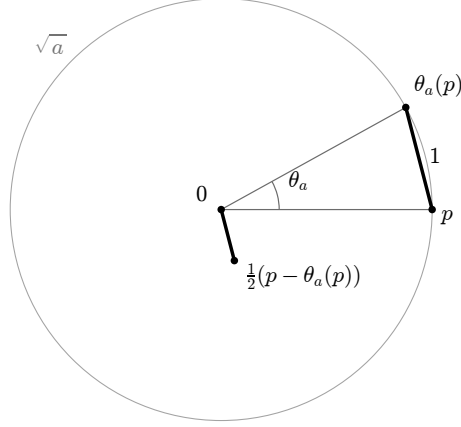
FIGURE 1. The spindle at squared radius a . Two shell points at distance \sqrt{a} are carried into each other by \theta_a and land at distance exactly 1, which is what the rotation is for. Half that displacement has length \frac{1}{2} always, since |1 - \theta_a| = 1/\sqrt{a} ; whether it lies in the lattice is the whole content of Theorem 1. Drawn for a = 4 , \cos \theta_4 = 7/8 .
