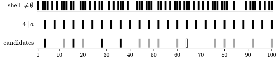
FIGURE 3. Theorem 1 as a sieve, over the integer spindles a \leq 100 . Top: the 59 positive squared radii at which R has points, decided by the form (3) rather than by a ball, and in closed form by Theorem 17. Middle: the multiples of 4. Bottom: their intersection, the sixteen multiples of 4 with an occupied shell—the candidates, in the sense Section 6 fixes. The nine gaps there are the multiples of 4 whose shell is empty, a = 8, 24, 32, 40, 56, 68, 72, 88, 96 ; they lie outside this accounting altogether, because at an empty shell Theorem 1 is silent in both directions. The law is a kill, not a construction, so the bottom row also carries what became of each candidate: filled, the four given a verified 5-chromatic union in Section 6; grey, the eleven the stronger filter of Section 7 kills; open, a = 64 , on which that filter degenerates at every modulus tried—it joins all the same, by Lemma 19, which builds a graph there rather than testing one.
