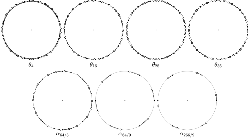
FIGURE 6. The seven joining rotations, each on its shell at radius \sqrt{a} : the lattice points at squared radius a (filled), their images under the rotation (open), and the unit edge every pair acquires. The shells hold 30, 30, 60, 54, 18, 6 and 6 points. Panels are drawn to a common circle size, so what varies across them is the shell and the rotation angle, not the scale; since |1 - \theta_a| = 1/\sqrt{a} the chord is 1 in every panel and the angle closes as a grows.
