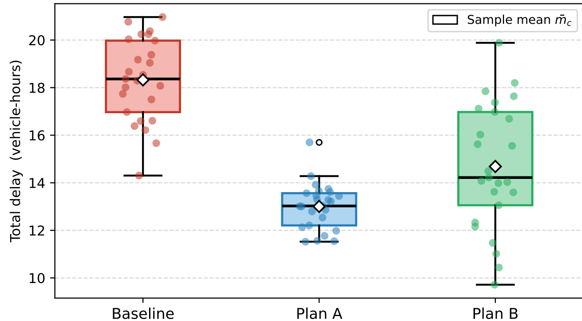
Distribution of total delay across R = 25 Monte Carlo runs
