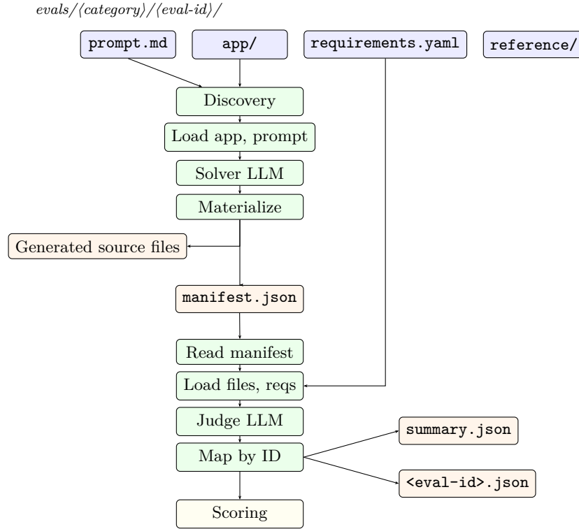
Figure 1: End-to-end pipeline of the React Native Evals benchmark. Dataset inputs (blue) feed the Generation CLI (described in section 3.3), producing manifest.json and source files generated by the solver. The Judge CLI (described in section 3.4) reads the manifest and requirements.yaml , runs the judge LLM, maps verdicts by requirement ID, and writes summary.json along with telemetry data. Scoring computes metrics as described in section 6.
