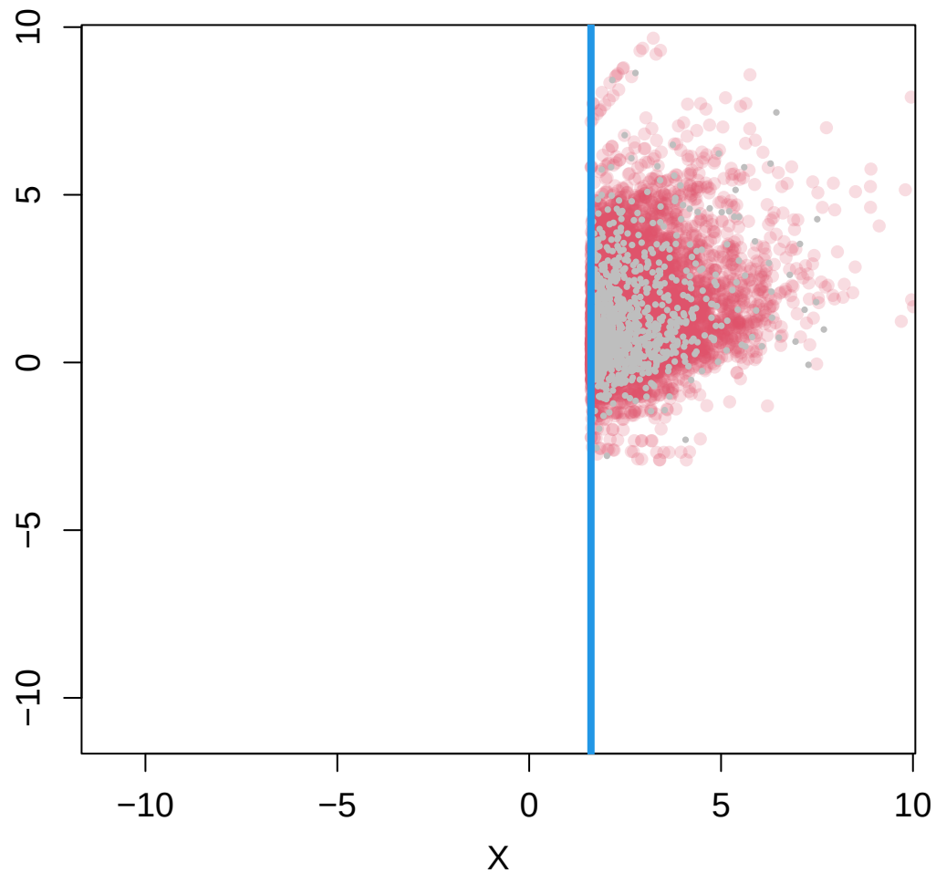
Conditional extremes simulations
