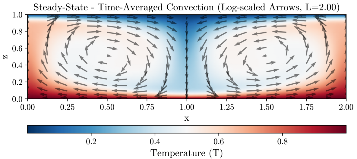
Figure 3.1: Example of a steady-state of a Rayleigh-Bénard system, with L = 2 - the arrows are log-scaled velocity vectors.
