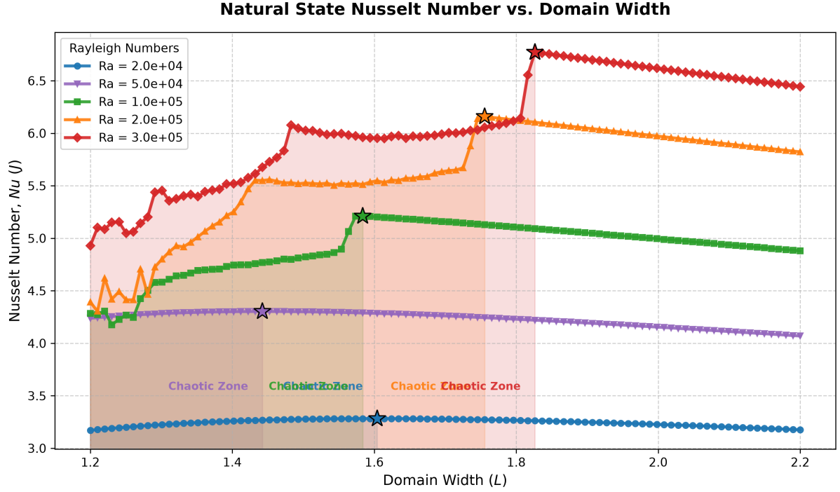
Figure 3.2: Plot of Nu against domain width, L , for Ra \in \{2 \times 10^4, 5 \times 10^4, 1 \times 10^5, 2 \times 10^5, 3 \times 10^5\}
