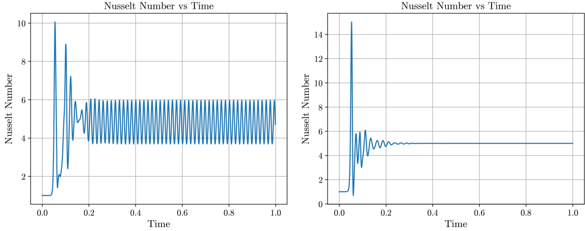
Figure 3.3: Plot of Nusselt number against time for L = 1.4 , Ra = 10^5 - chaotic zone. Figure 3.4: Plot of Nusselt number against time for L = 2.0 , Ra = 10^5 - stable zone
