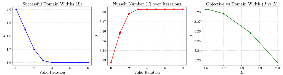
Figure 3.5: Optimisation results using the adjoint-based method with L_0 = 2.0 , Ra = 2 \times 10^4 , Pr = 1
