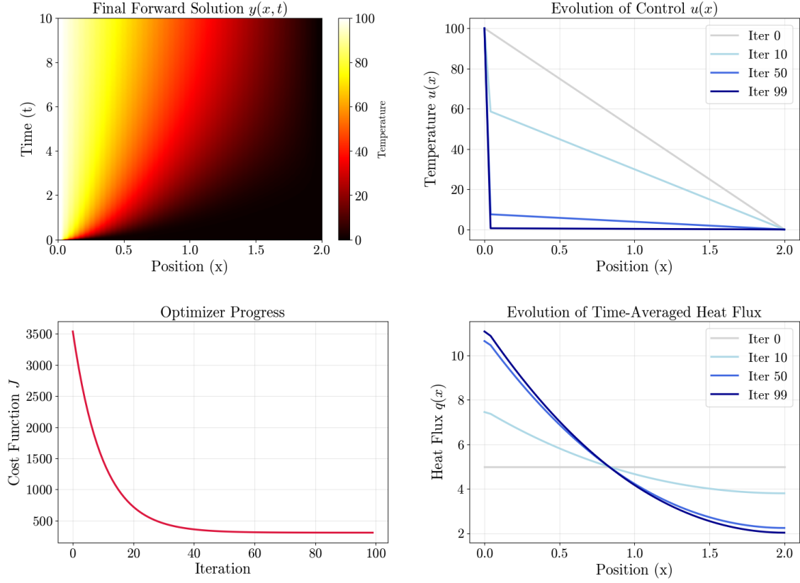
Figure 2.1: Two-Dimensional Adjoint Optimisation Results
