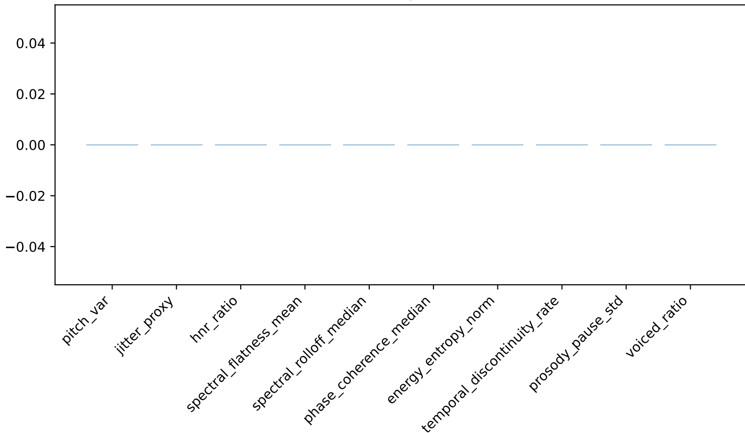
Feature Importance
