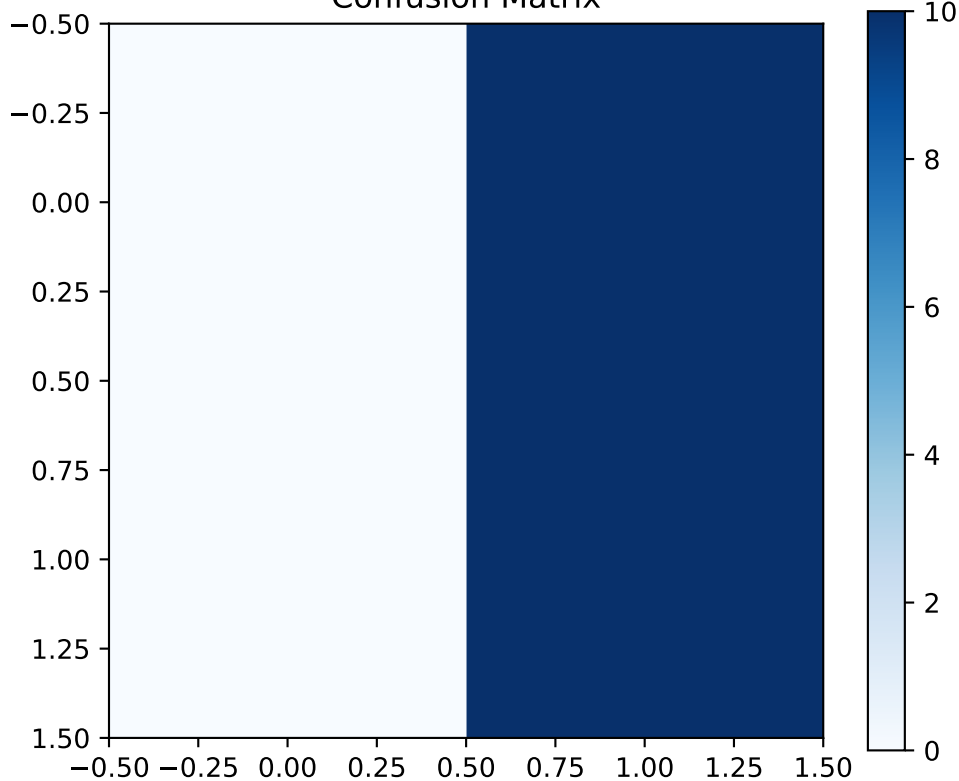
Confusion Matrix
