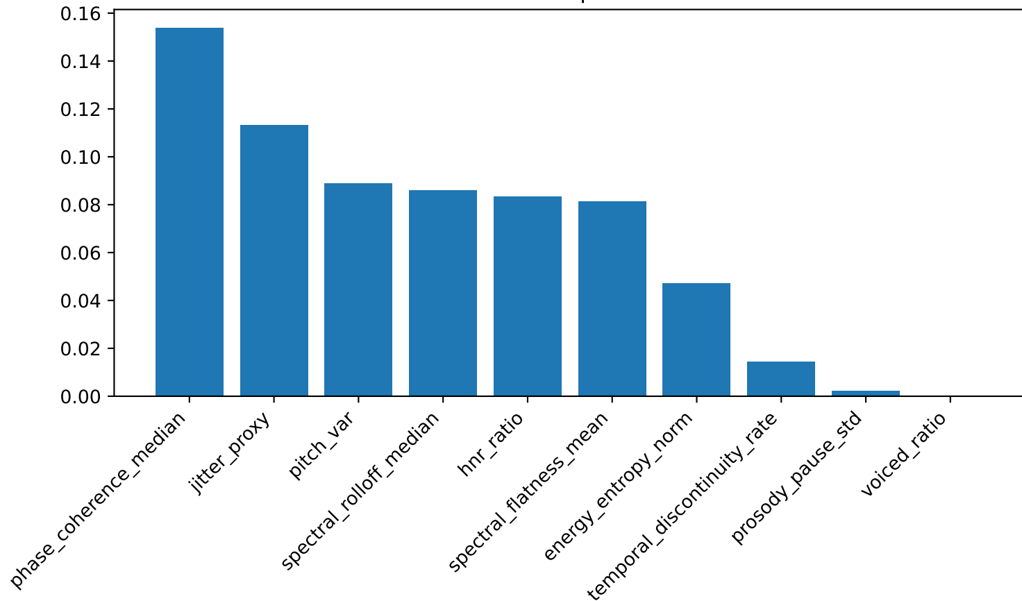
Feature Importance
