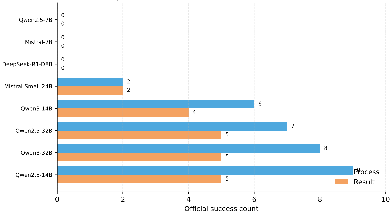
Comparable local cohort under GitTaskBench official metrics
