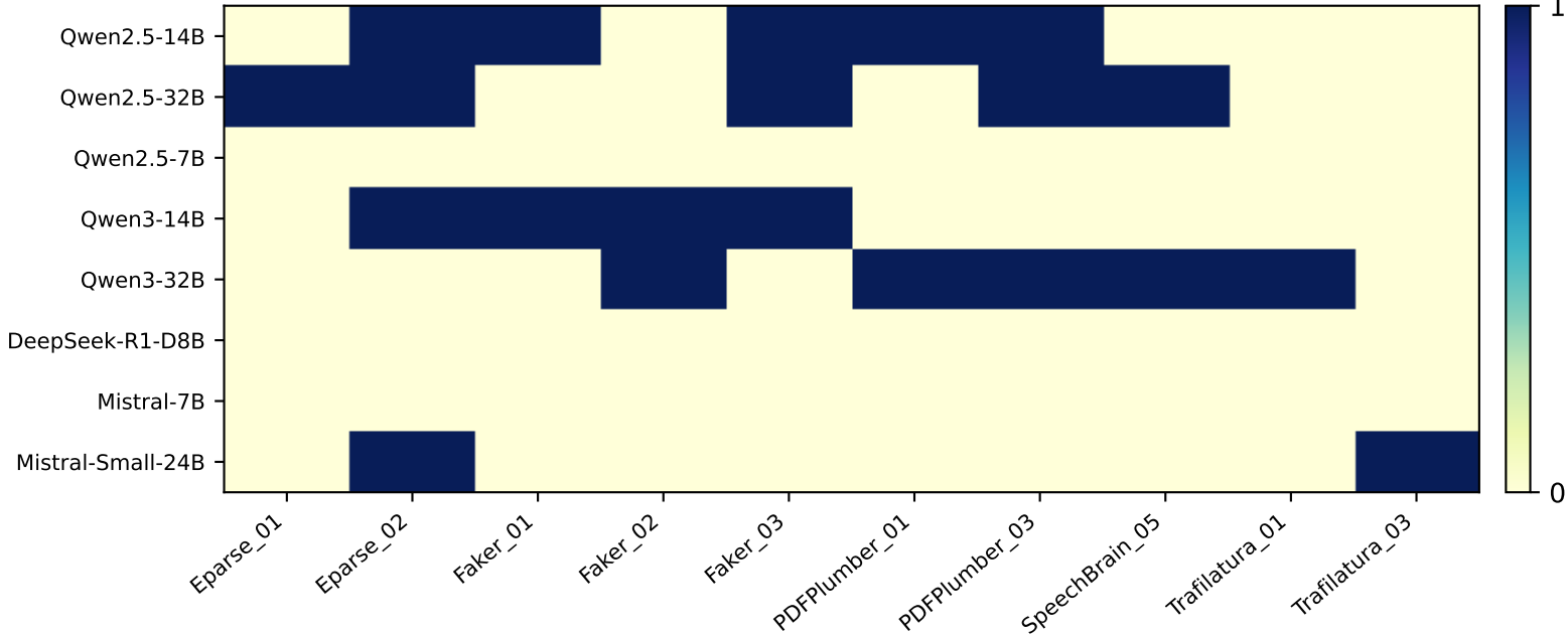
Tied headline scores still hide task-family specialization
