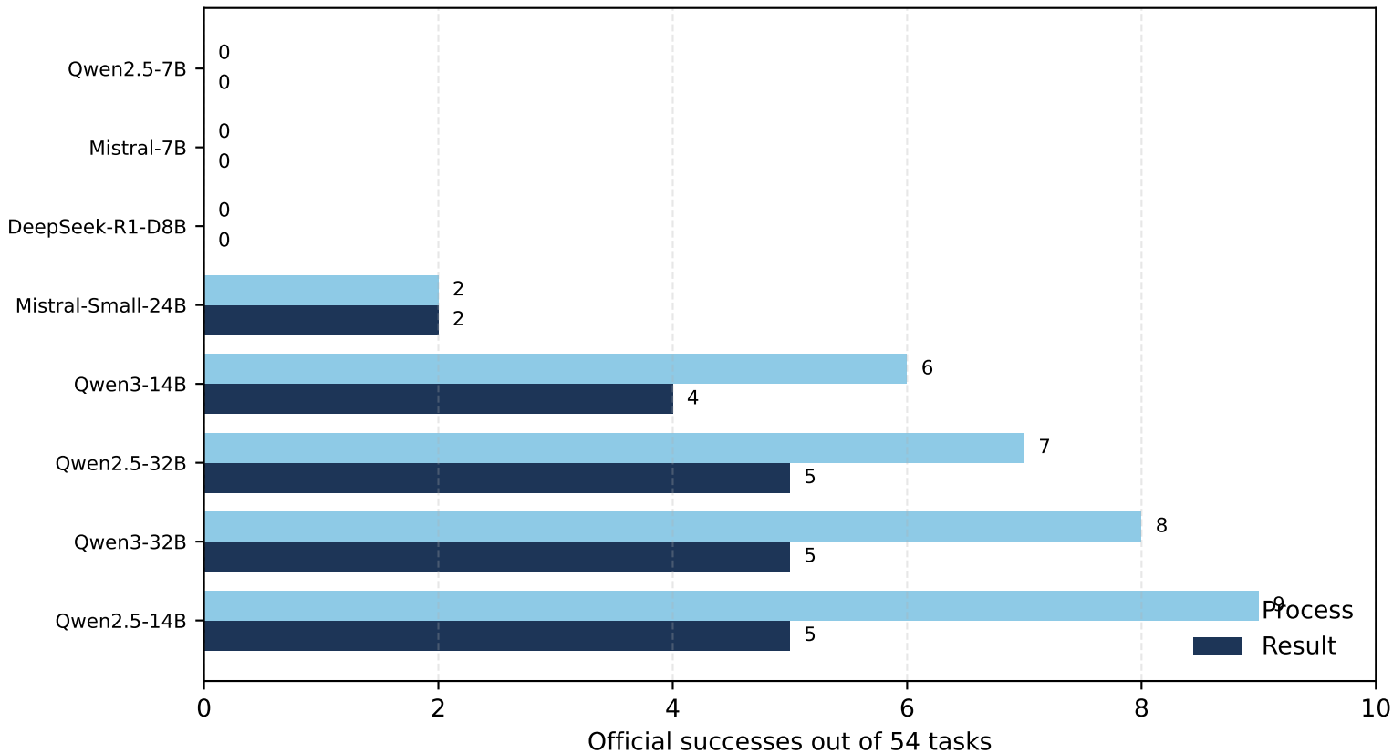
Comparable open-8 cohort under GitTaskBench official metrics
