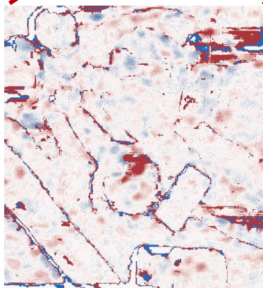
D435 depth deviation
