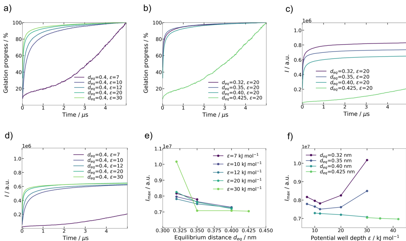
Figure 7. (a) Virtual gelation progress ( I/I_{\max} in %) for constant d_{\text{eq}} = 0.4 nm, (b) virtual gelation progress ( I/I_{\max} in %) for constant \epsilon = 20 kJ mol ^{-1} , (c) intermolecular interactions ( I ) between glucose repeating units of the cellulose polymer chains during gelation simulation for constant \epsilon = 20 kJ mol ^{-1} , (d) intermolecular interactions ( I ) between glucose repeating units of the cellulose polymer chains during gelation simulation for constant \epsilon = 20 kJ mol ^{-1} , (e) maximum intermolecular interactions I_{\max} between glucose repeating units of the cellulose polymer chains at \tau = 5 \mu s as a function of d_{\text{eq}} , and (f) maximum intermolecular interactions I_{\max} between glucose repeating units of the cellulose polymer chains at \tau = 5 \mu s as a function of \epsilon .
