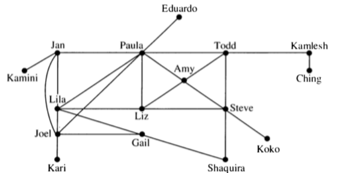
FIGURE 7 An Acquaintanceship Graph.
