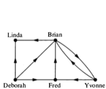
FIGURE 8 An Influence Graph.
