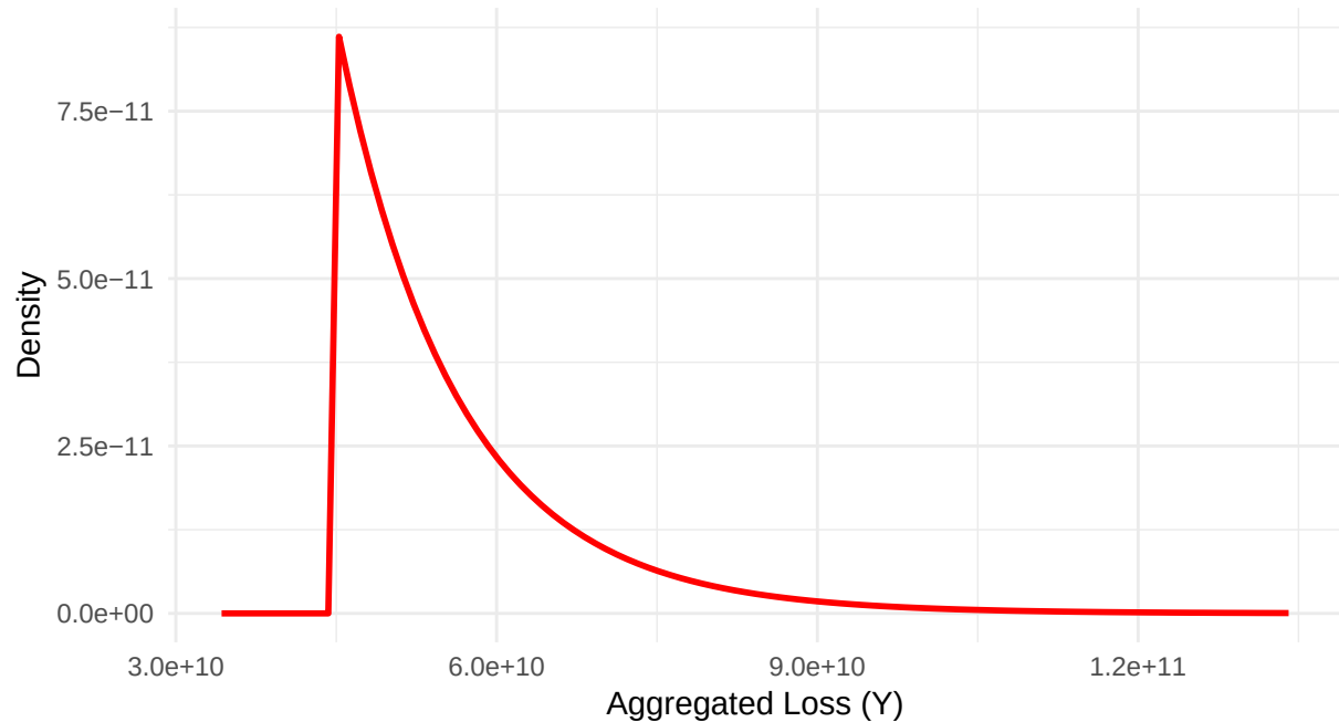
Aggregated Loss Distribution with GPD Tail Fit
