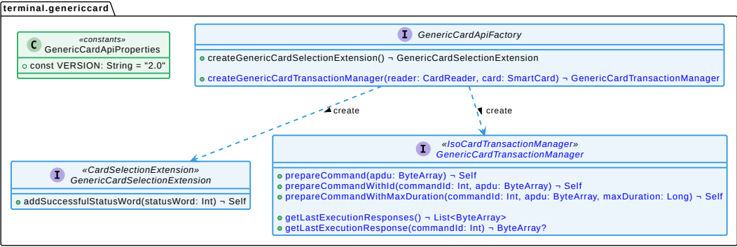
Figure 2. Terminal Generic Card API—UML Class Diagram
