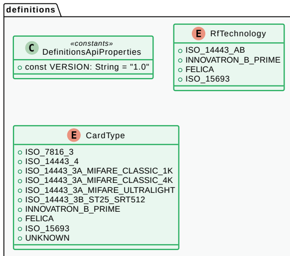
Figure 2. Terminal Definitions API—UML Class Diagram
