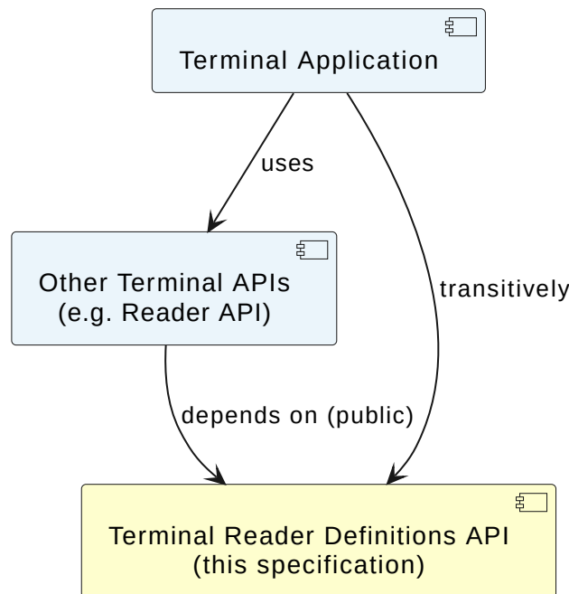
Figure 1. Terminal Reader Definitions API—Architecture Overview
