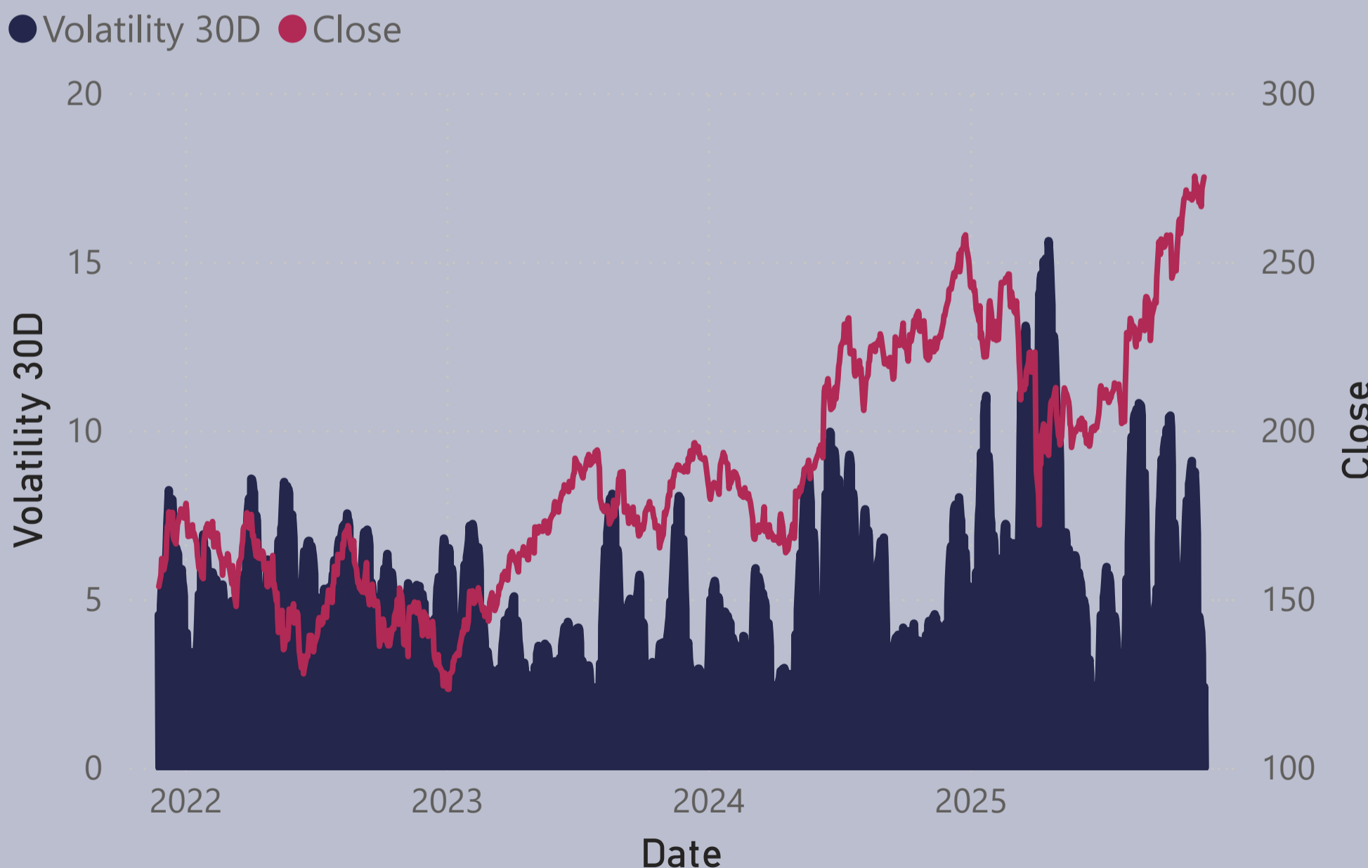
Volatility 30D and Close by Date
