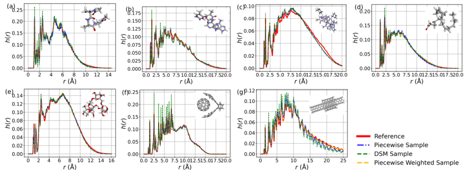
Figure 3: The distribution of interatomic distances ( r (Å)) for (a) Ac-Ala3-NHMe, (b) DNA base pair (AT-AT), (c) DNA base pair (AT-AT-CG-CG), (d) Docosaehaenoic acid, (e) Stachyose, (f) Buckyball catcher, (g) Dw nanotube in MD22 dataset. The insets display the ball-and-stick representations of these molecules.
