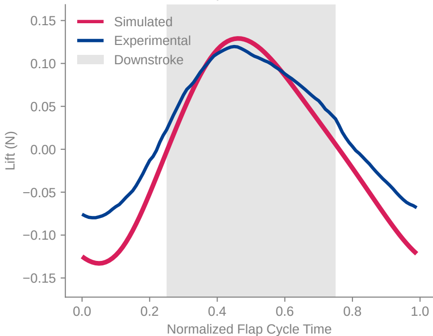
Simulated and Experimental Lift Versus Time
