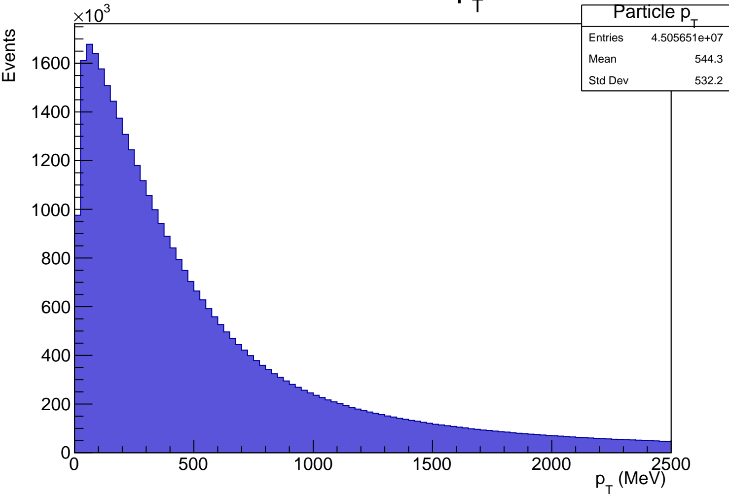
Plot 4: Particle p_T
