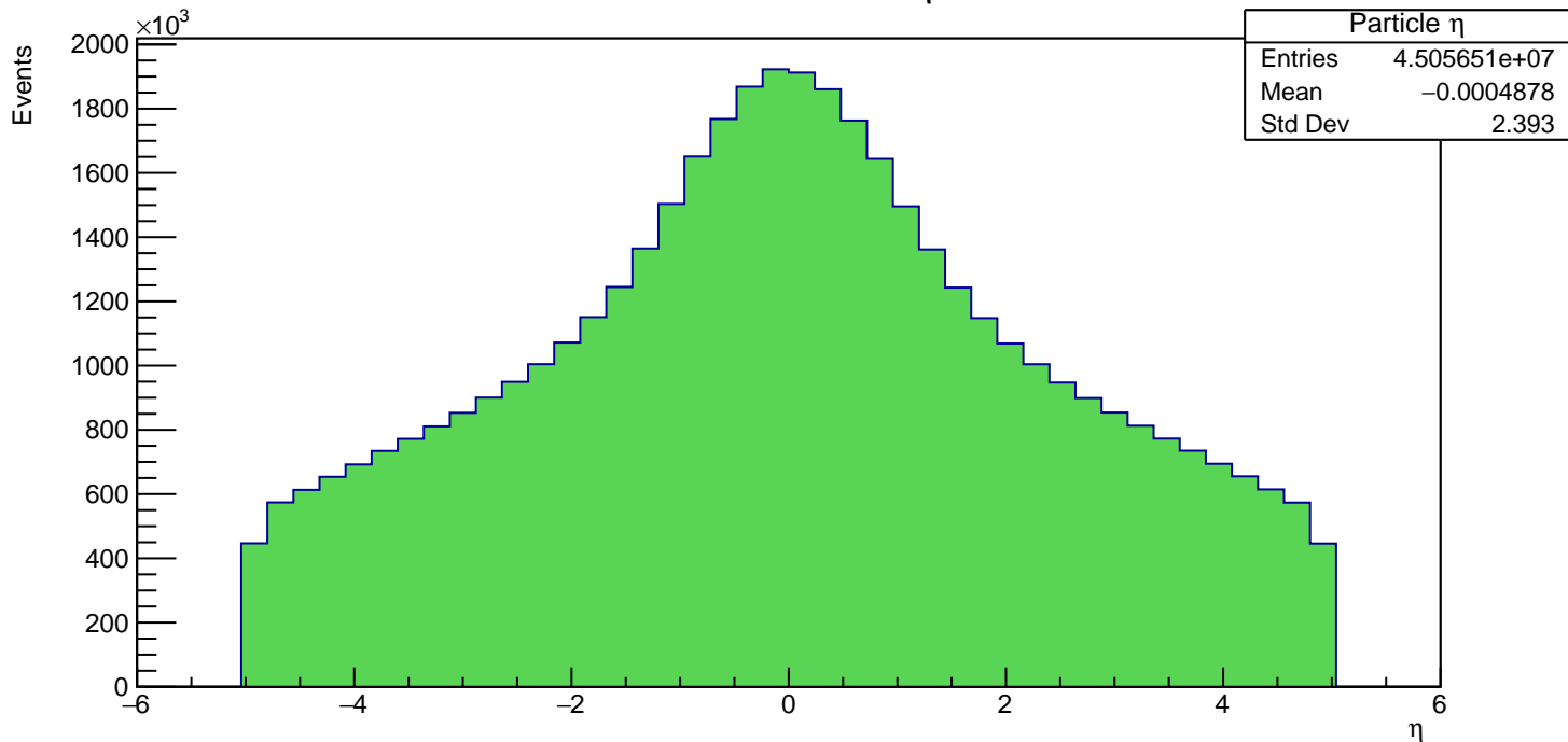
Plot 4: Particle \eta
