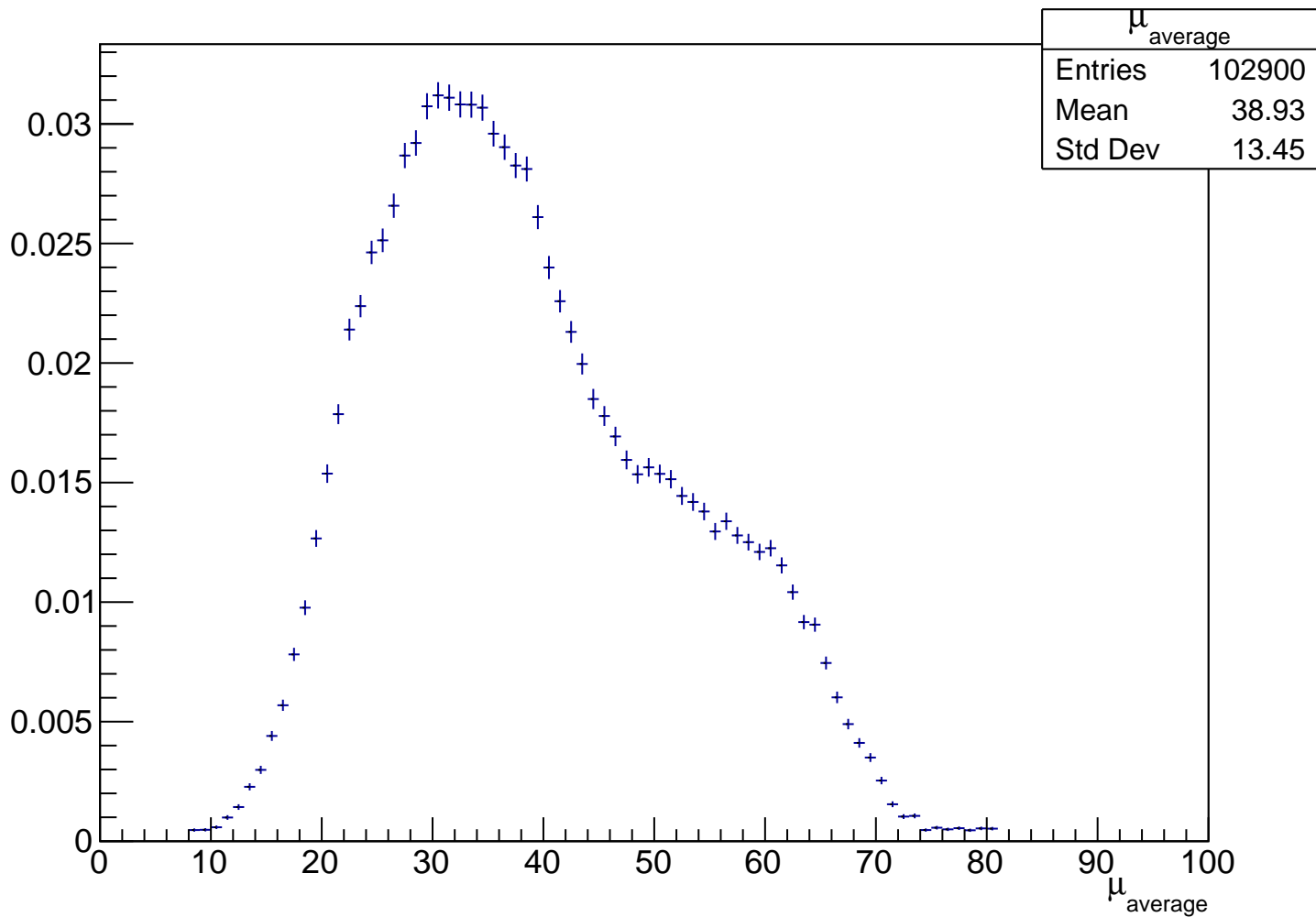
Plot 1: Number of average interactions per bunch-crossing
