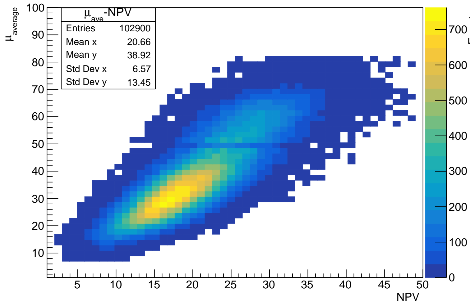
Plot 2: 2D Histogram Numbers of events vs. \mu_{\text{average}} and NPV
