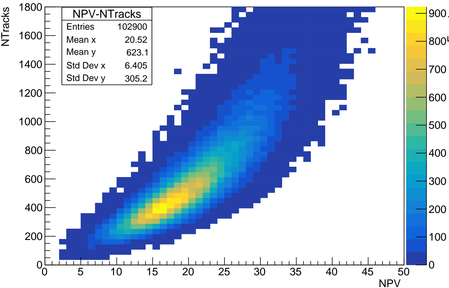
Plot 3.1: Number of events vs. NPV and NTracks
