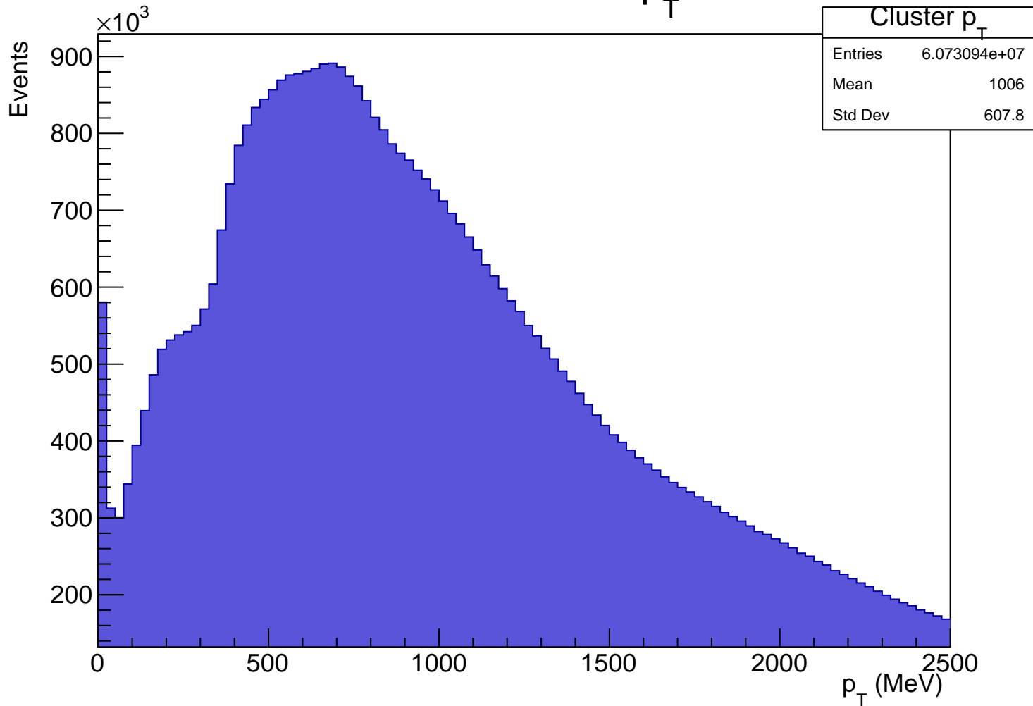
Plot 4: Cluster p_T
