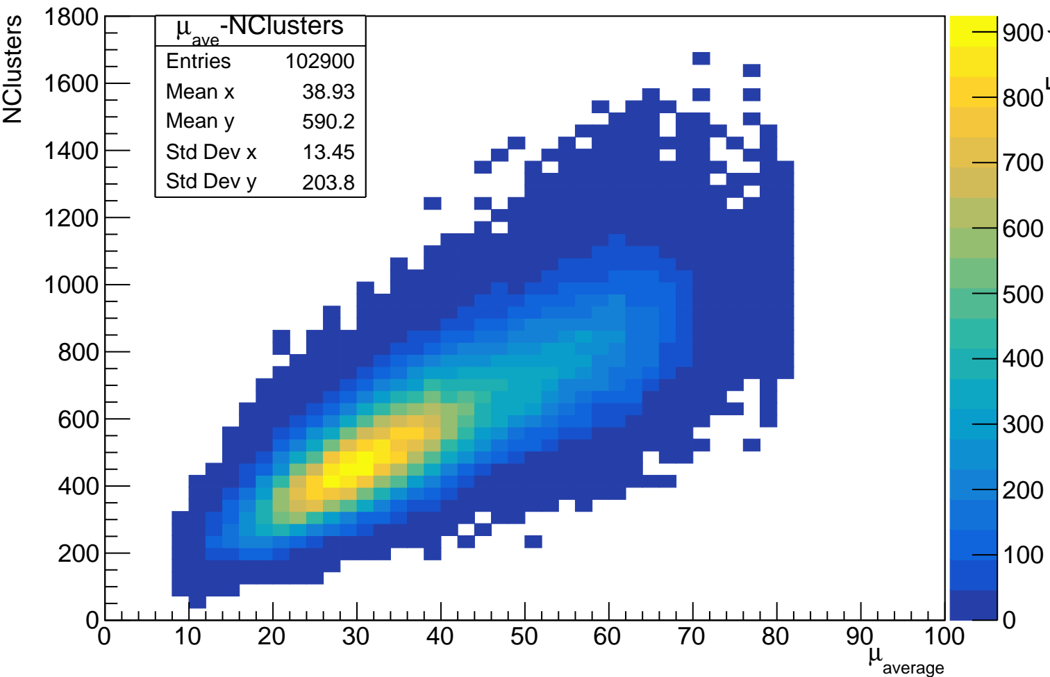
Plot 3.4: Number of events vs. \mu_{\text{average}} and NClusters
