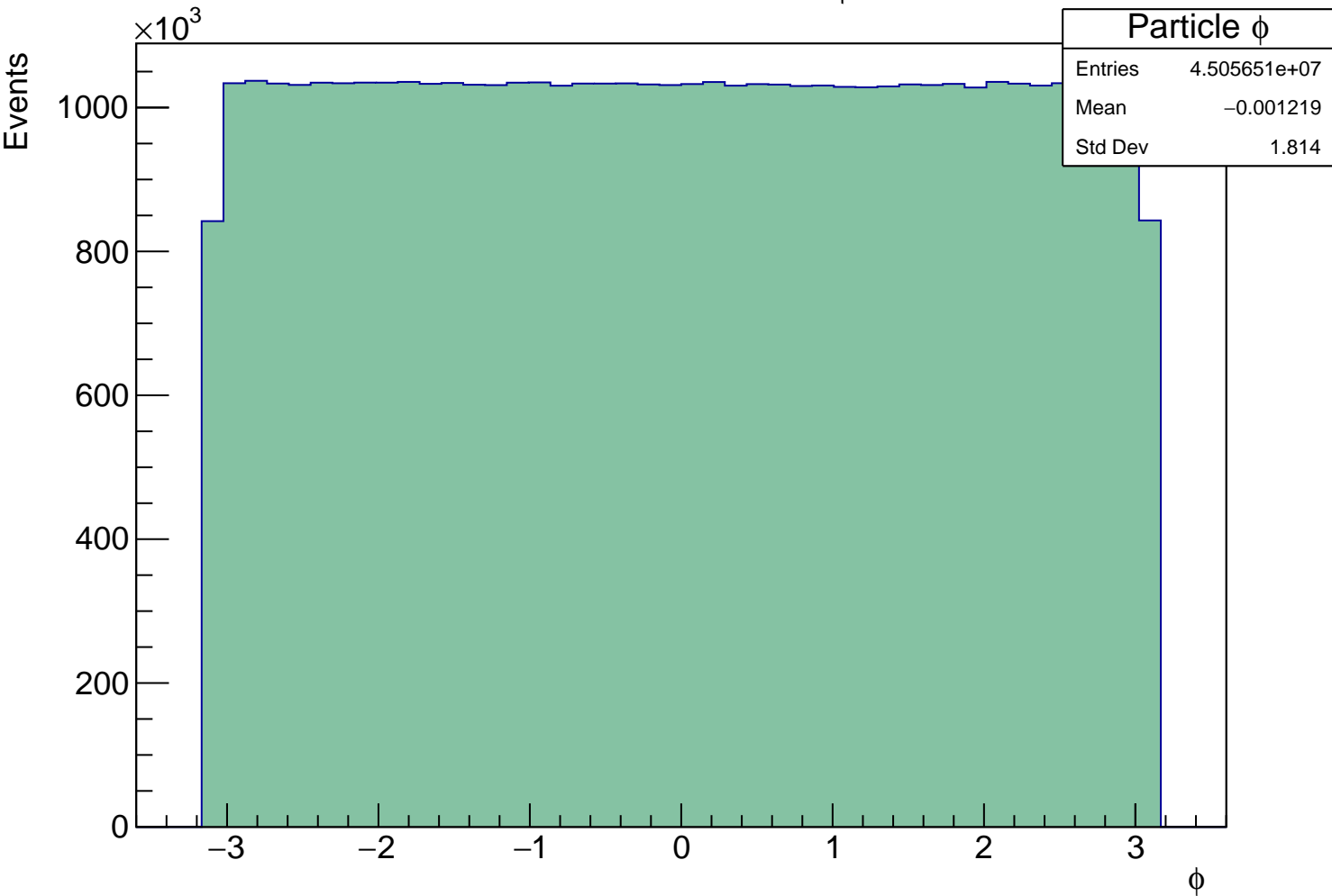
Plot 4: Particle \phi
