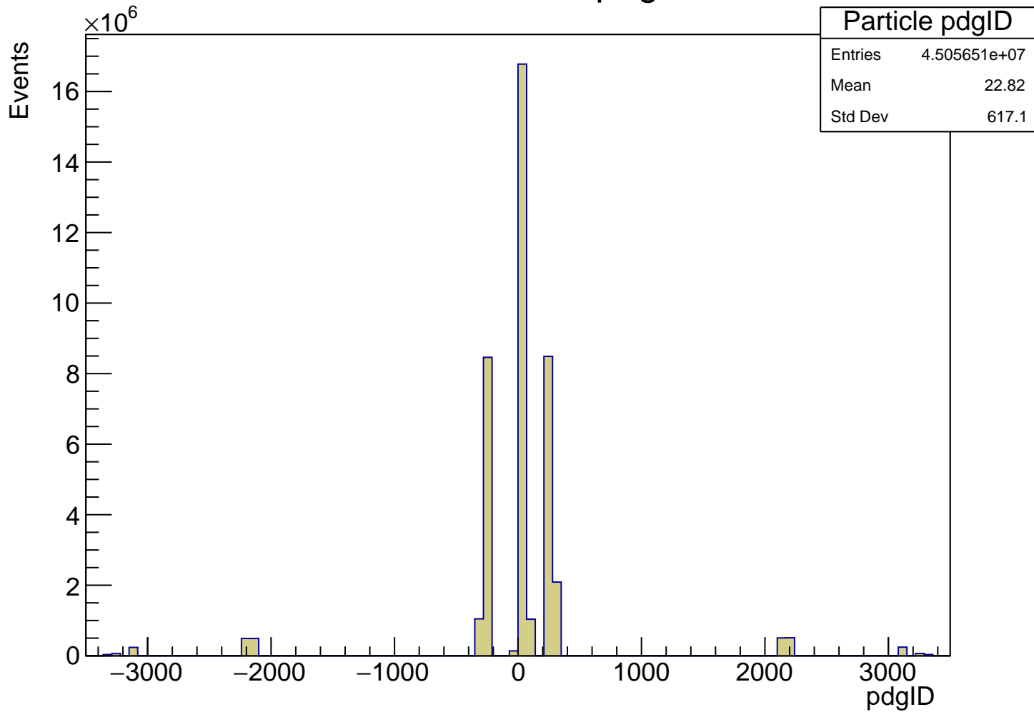
Plot 4: Particle pdgID
