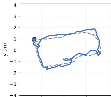
Cambrian-P (Ours)
