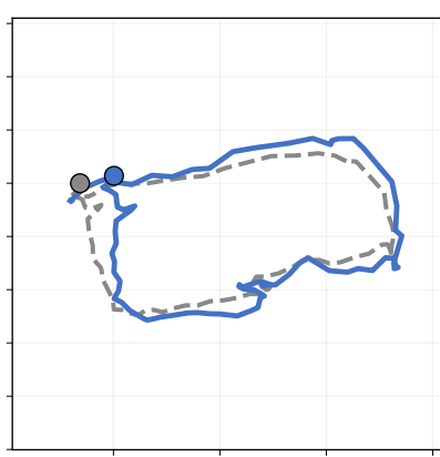
CUT3R
