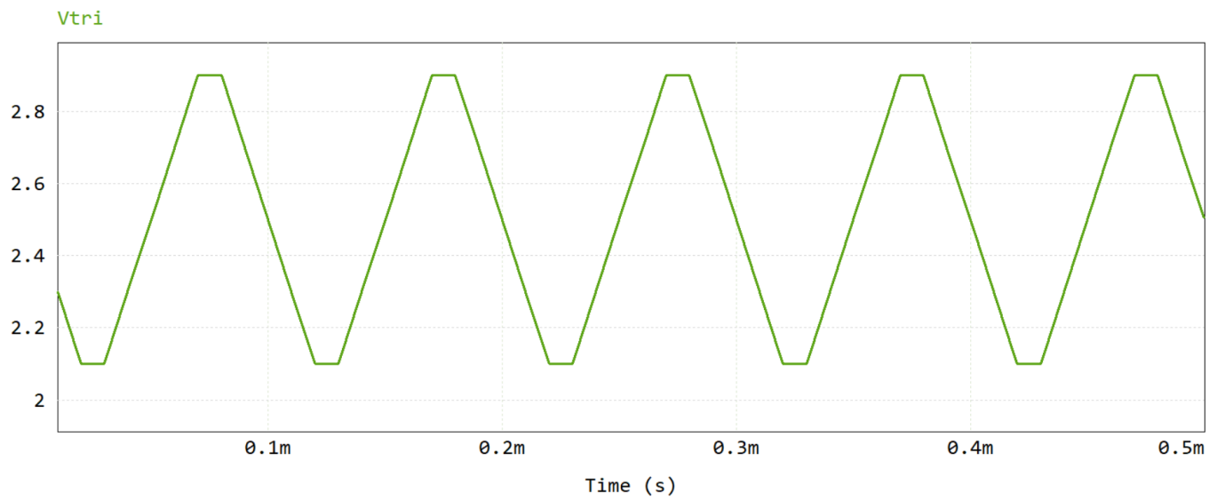
Fig. 12. Triangular-wave voltage with the total simulation time reduced to below 10 cycles.
