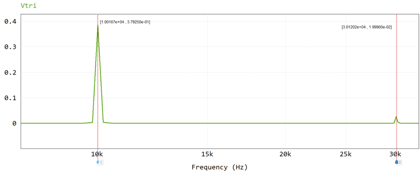
Fig. 14. FFT of the triangular-wave voltage with the total simulation time increased to more than 10 cycles. Cursors mark the fundamental (10.02 kHz, 0.379) and the third harmonic (30.12 kHz, 0.020).
