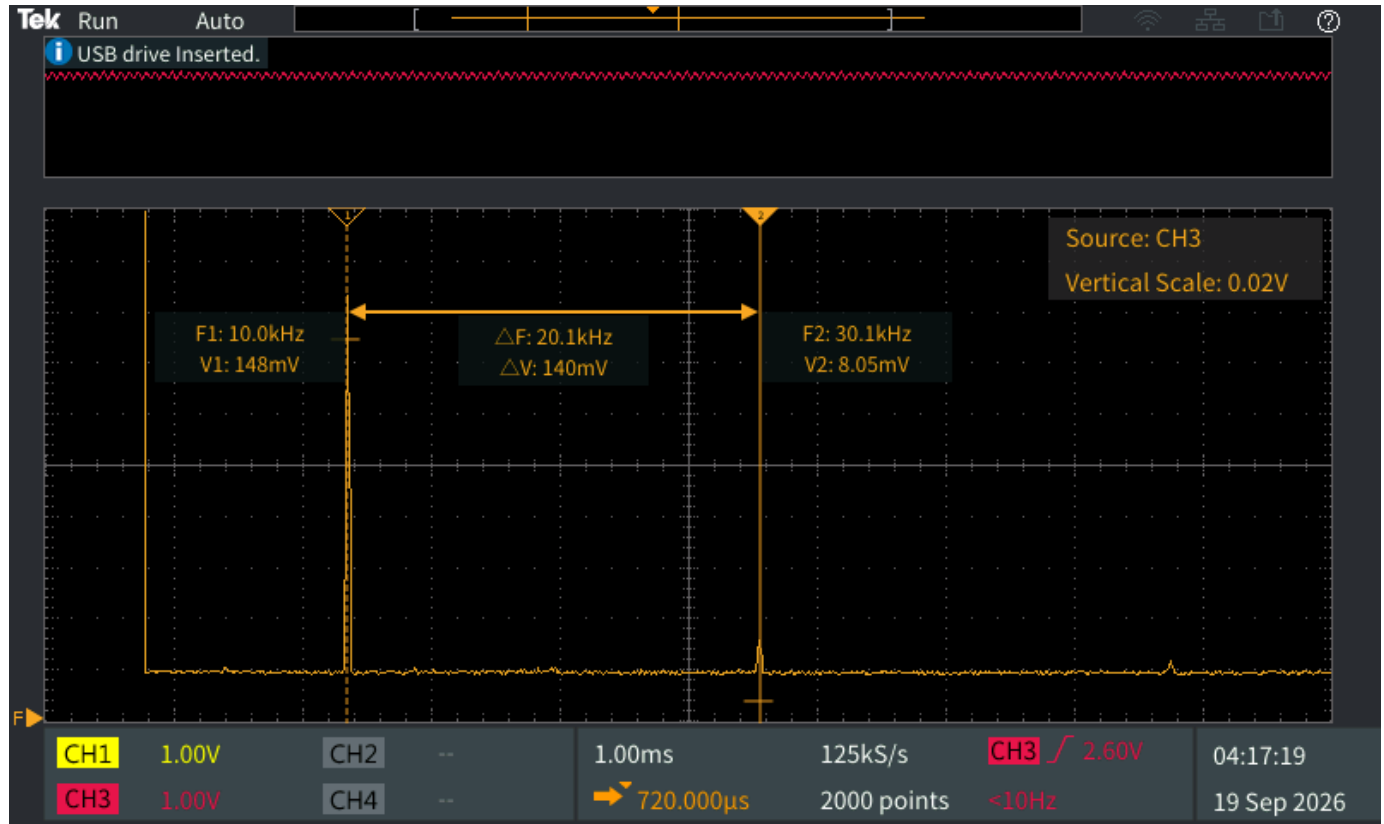
Fig. 19. FFT of the 10 kHz triangular wave.
