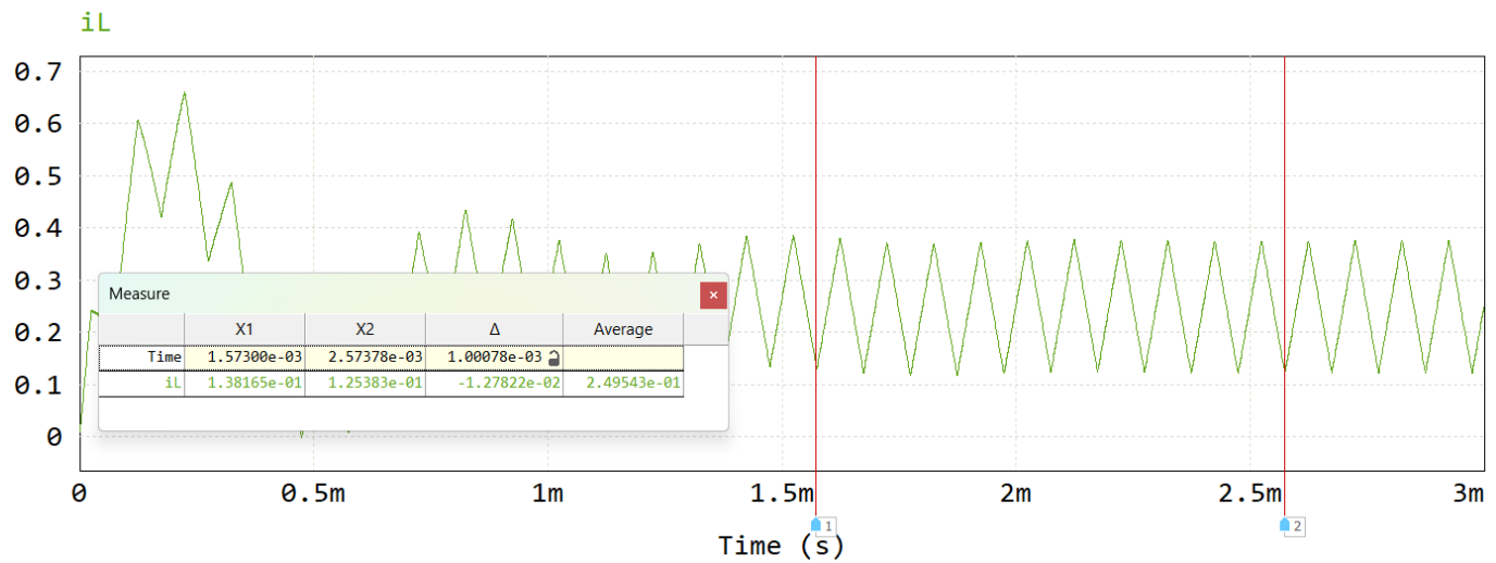
Fig. 9. Mean-value measurement of i_L over 10 steady-state cycles (1.00 ms).
