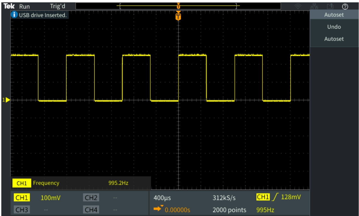
Fig. 16. Differential probe: oscilloscope capture of the calibration signal.
