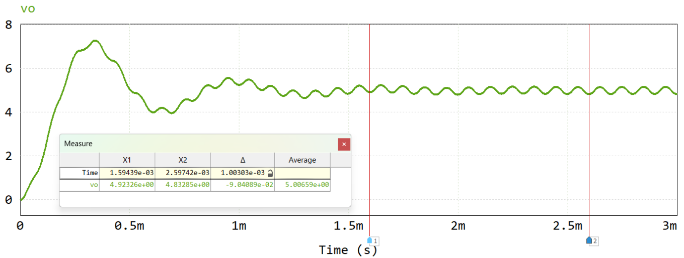
Fig. 8. Mean-value measurement of v_o over 10 steady-state cycles (1.00 ms).
