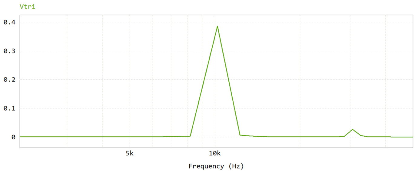
Fig. 13. FFT of the triangular-wave voltage with the total simulation time reduced to below 10 cycles.
