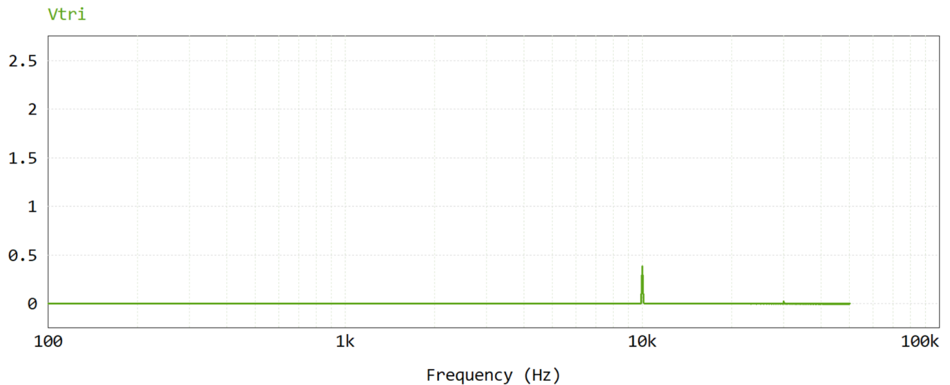
Fig. 11. FFT of the triangular-wave voltage, full span.
