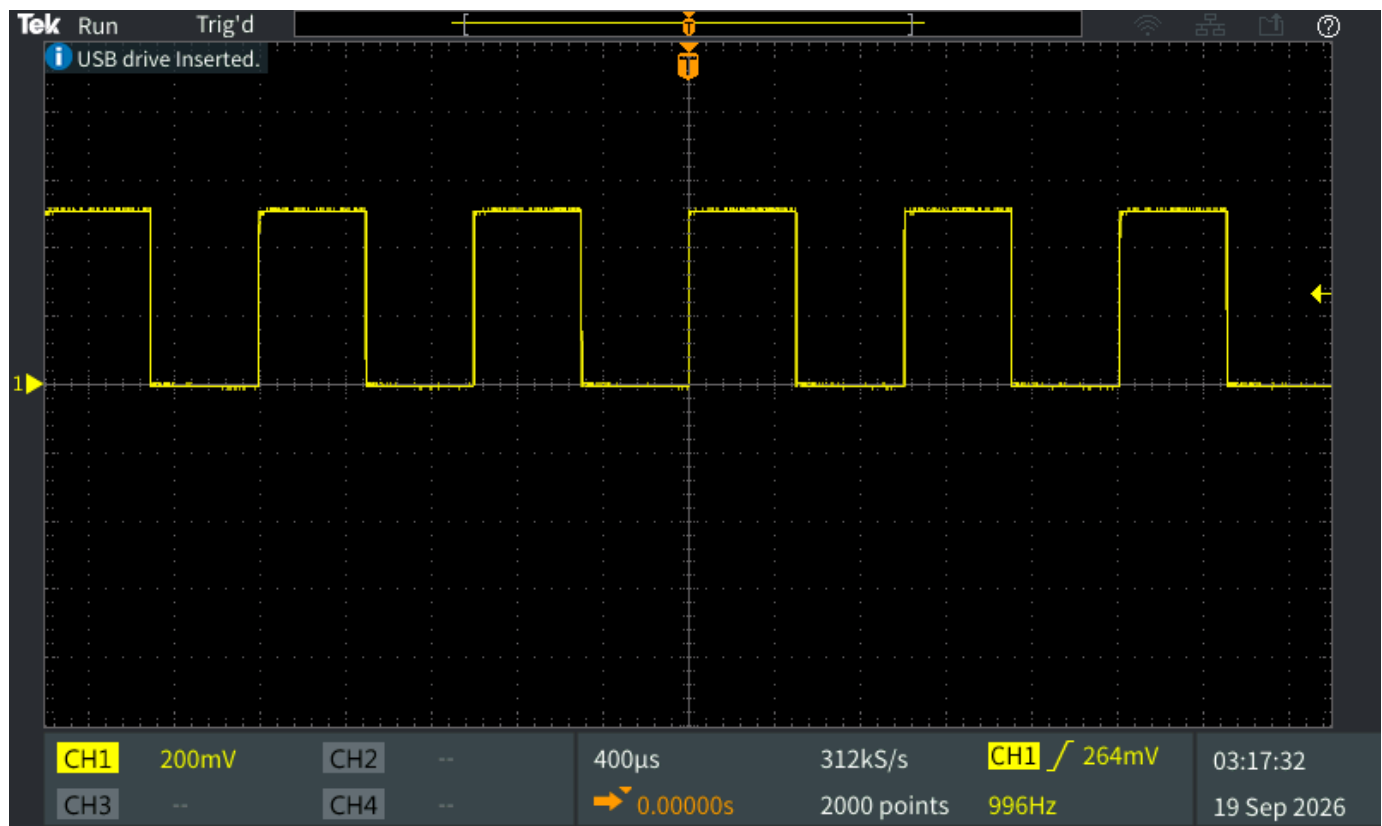
Fig. 15. Passive probe: oscilloscope capture of the calibration signal.
