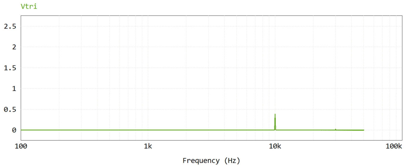
Fig. 11. FFT of the triangular-wave voltage, full span.
