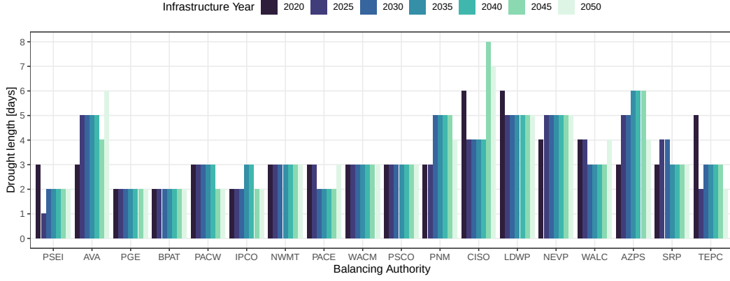
Figure 5. Maximum compound VRE drought duration for the net-zero high renewable scenario, which involves a fully decarbonized high renewable grid by 2050. Note that the figure does show boxplots, but in most BAs the distribution of drought duration is heavily skewed such that most boxes are collapsed on at the lowest value.
