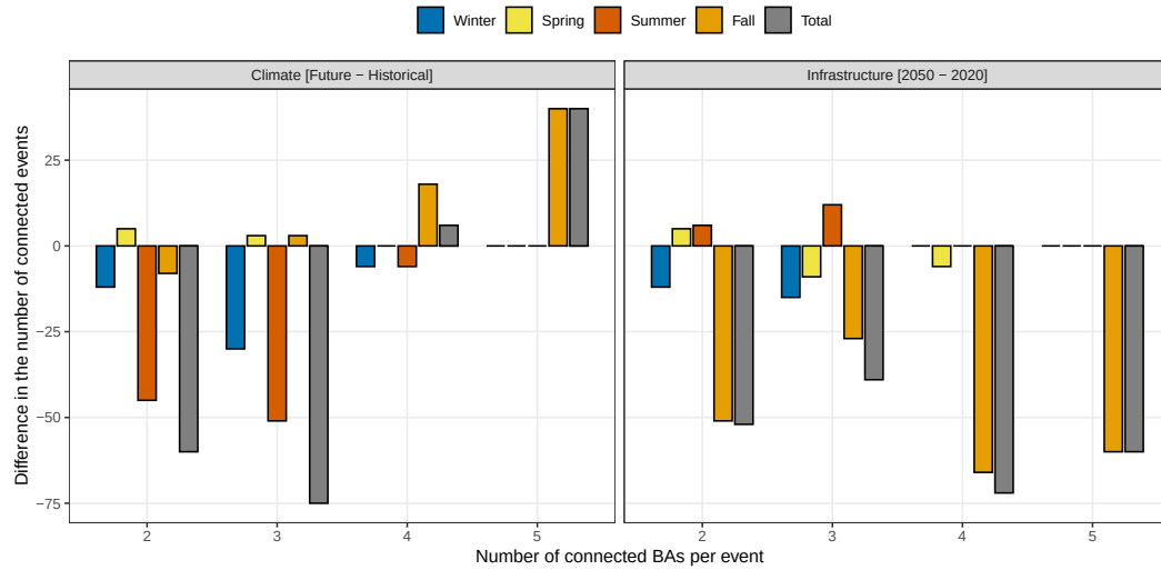
Figure 7. The difference between the number of multi-BA compound energy droughts in each season for the net-zero-high renewable scenario. The left panel shows the climate influence by differencing the future weather and historical weather periods using 2050 infrastructure. The right panel shows the infrastructure influence by differencing the 2050 and 2020 infrastructure scenarios both using future weather. Negative values indicate fewer connected events in the future period.
