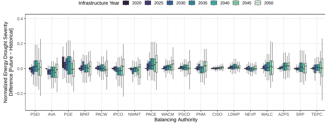
Figure 4. Difference in average annual normalized energy drought severity between the future and historical periods for the net-zero-high renewable scenario, which involves a fully-decarbonized high renewable grid by 2050. Severity has been normalized per BA to allow the data to be compared across BAs.
