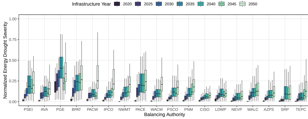
Figure 3. Energy drought severity (energy deficit below the 10th percentile) for the net-zero high renewable scenario which involves a fully-decarbonized-high renewable grid by 2050. Climate variability is simulated for each infrastructure year using 40-years of rcp85hotter climate forcing. Severity has been normalized by the maximum value in each BA to allow the data to be compared across BAs and outliers have been removed for visual clarity.
