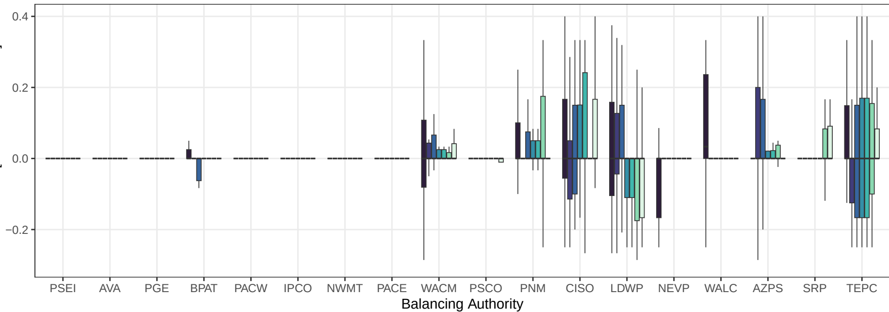
Normalized Energy Drought Severity Difference [Future - Historical]
