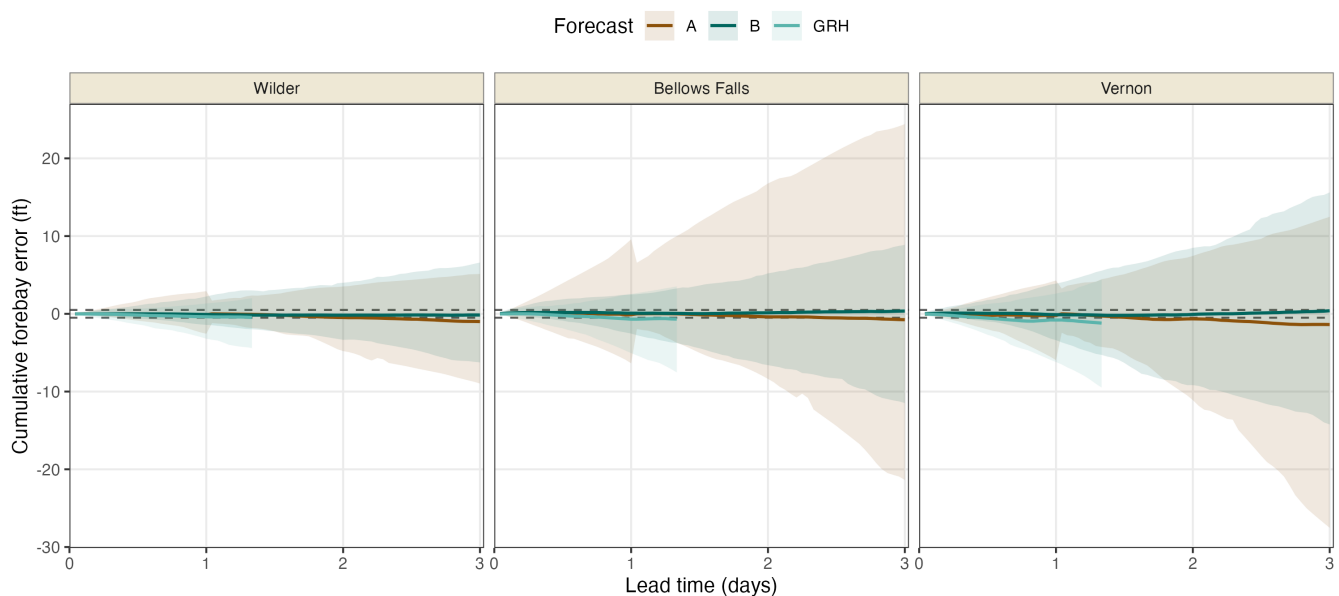
FIGURE 5 The cumulative probability of exceeding Cumulative forebay error under an idealized pass-inflow stress test with a 0.5-foot operating range if neutral starting position. Lines show the operations were set median across forecast issues and shaded bands span the 2.5th to pass-inflow-97.5th percentiles. Dashed lines mark the \pm 0.5 foot (inflow=outflow \approx 15 cm) where inflow was determined by the various inflow forecasts forebay operating band.
