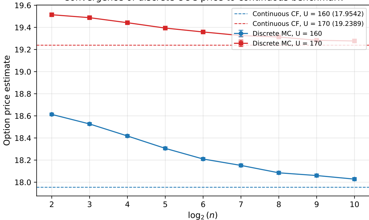
Convergence of discrete UOC price to continuous benchmark
