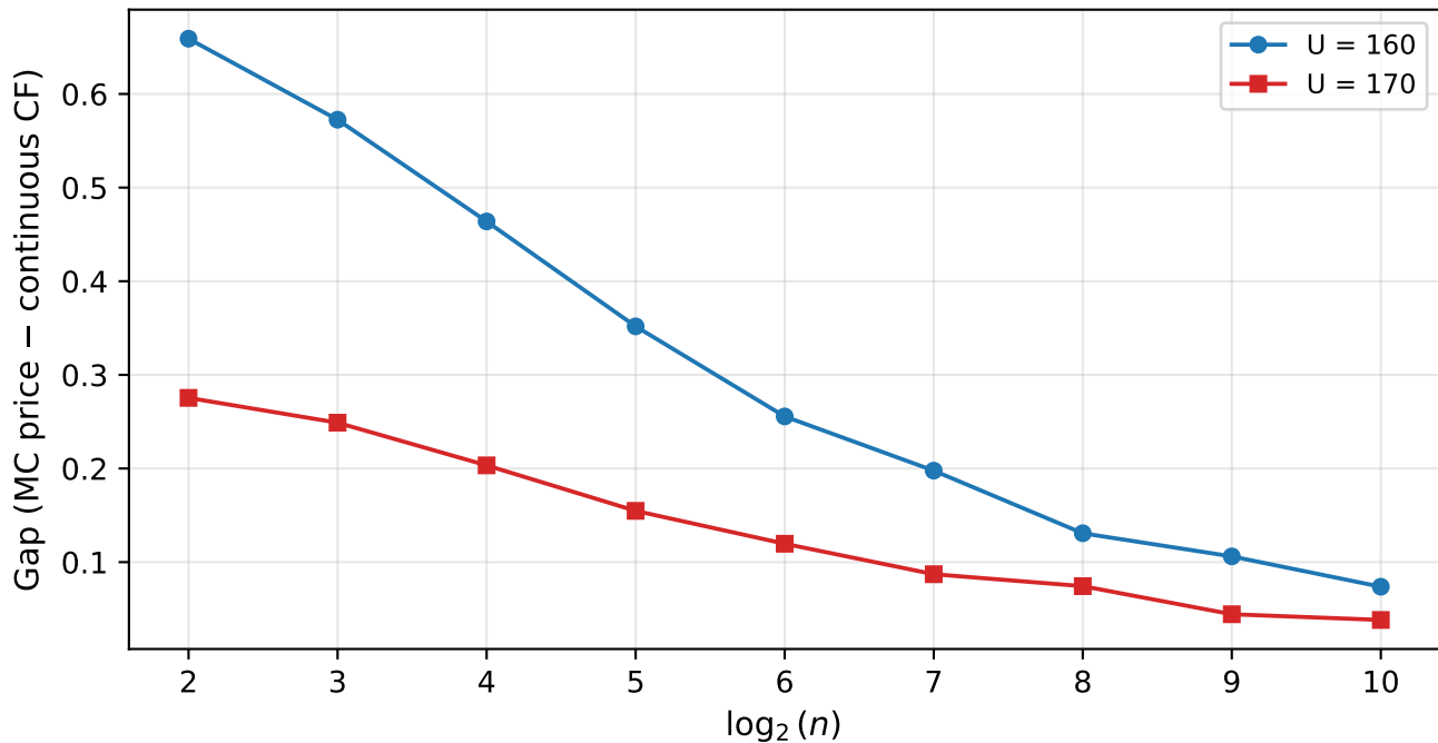
Discretisation gap vs. number of monitoring dates
