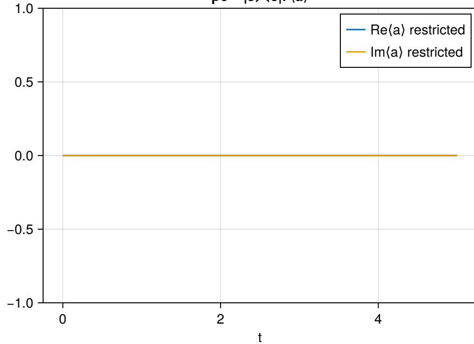
\rho_0 = |3\rangle\langle 3| : \langle a \rangle
