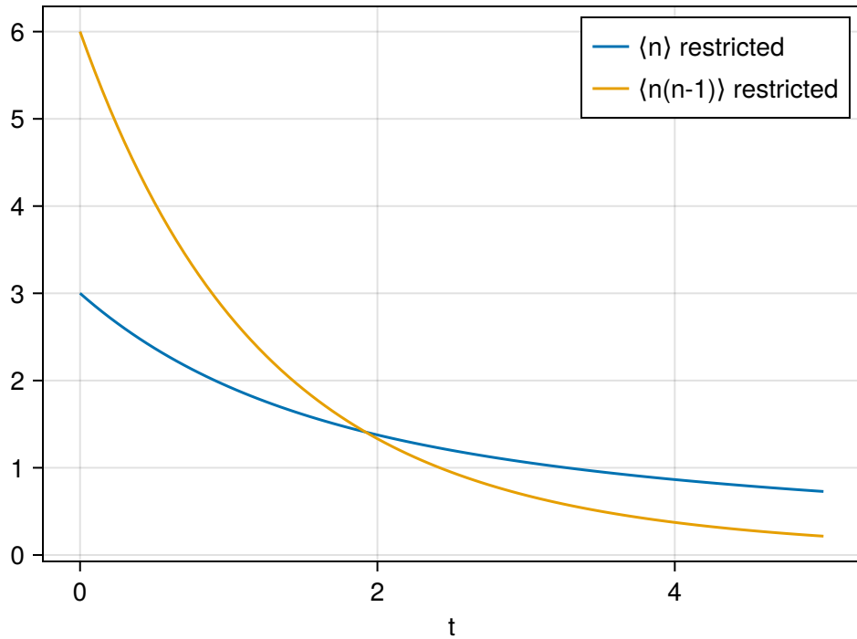
\rho_0 = |3\rangle\langle 3| : populations
