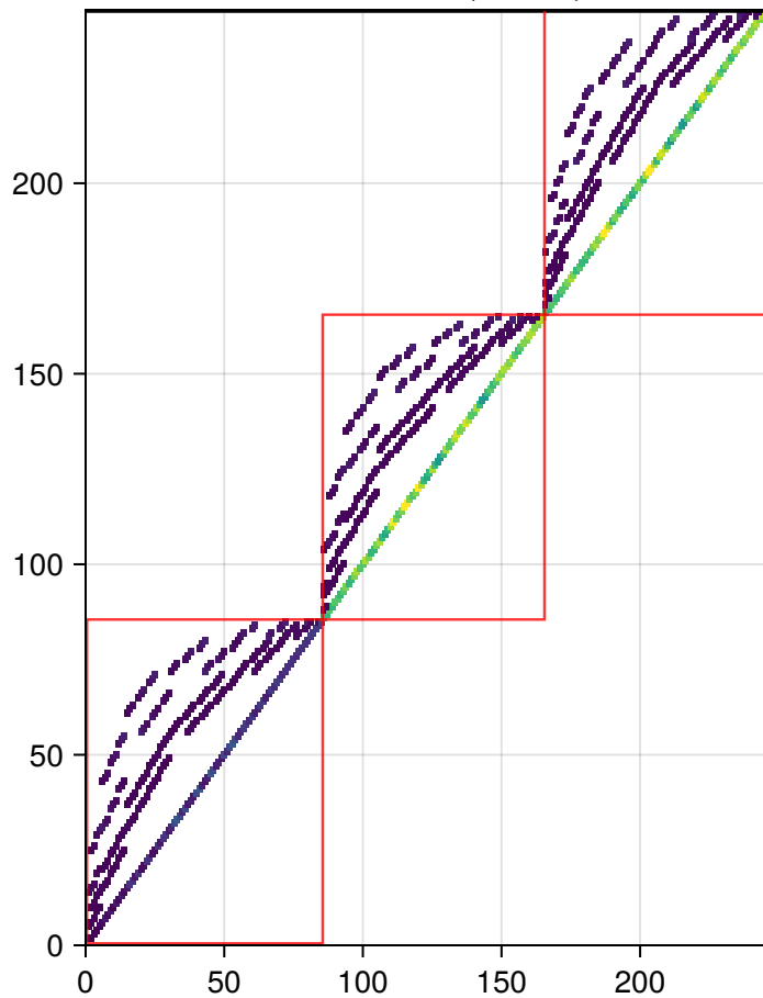
\mathcal{L} restricted (2 sites)
