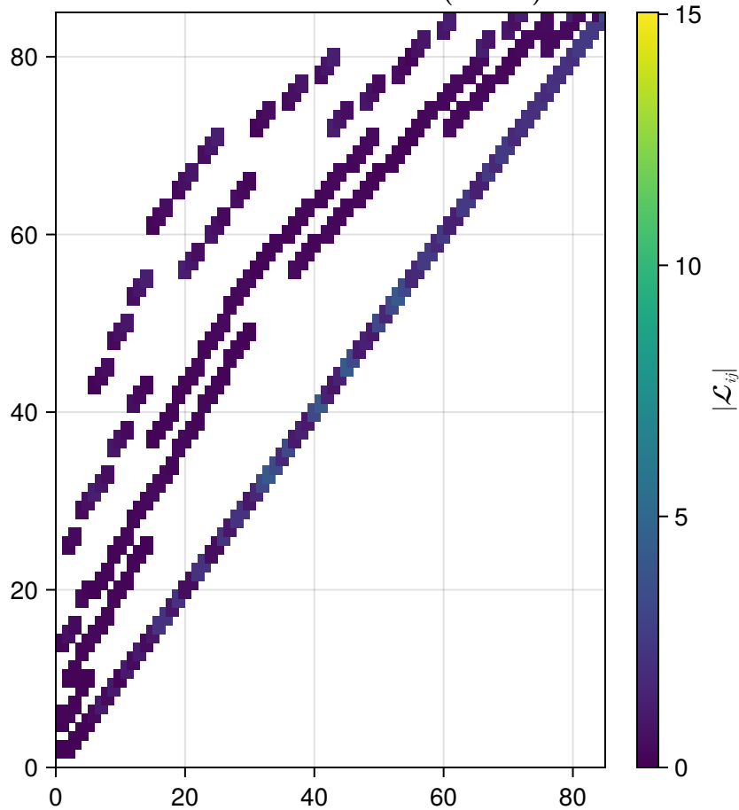
\mathcal{L} restricted: sector k=0 (2 sites)
