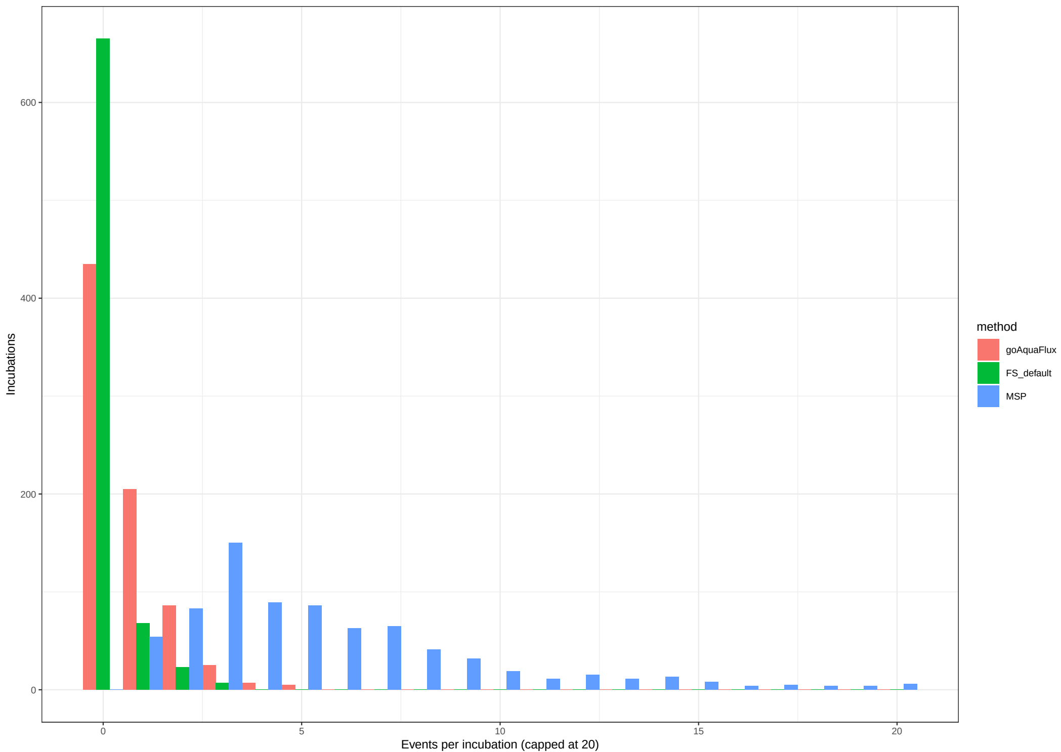
Number of detected ebullition events
