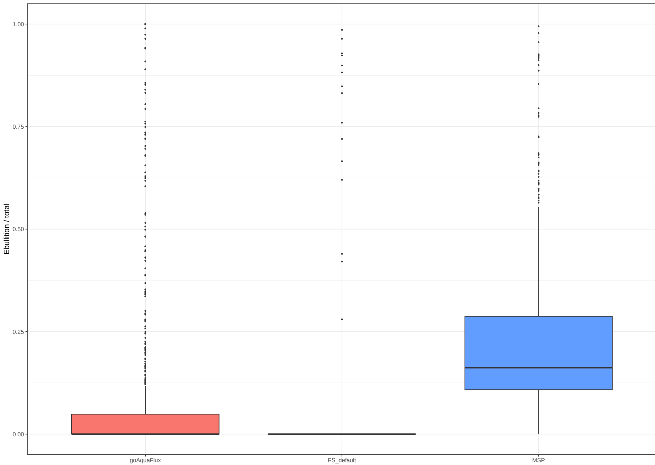
Ebullition fraction
