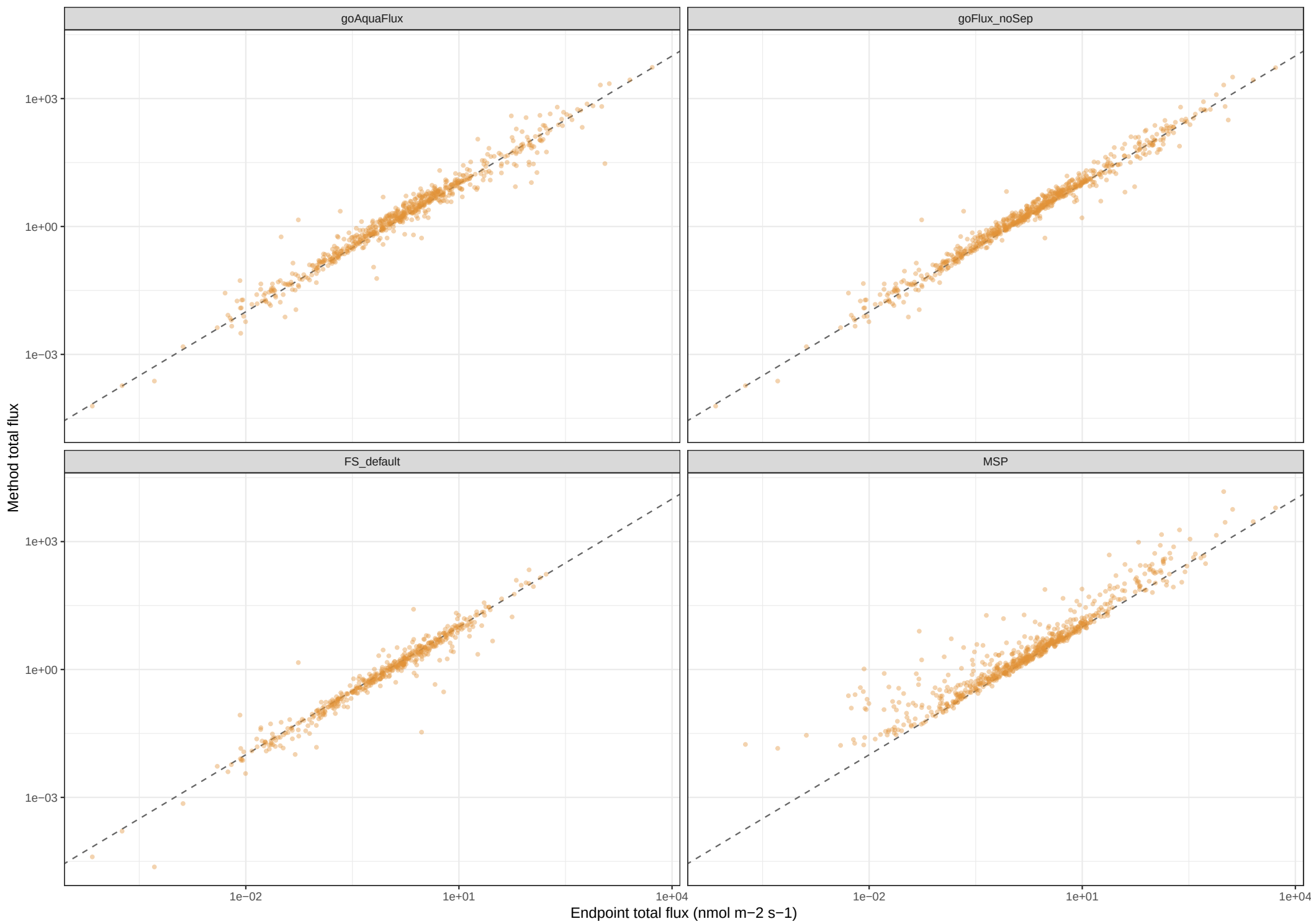
Total CH 4 flux vs model-free endpoint estimate
