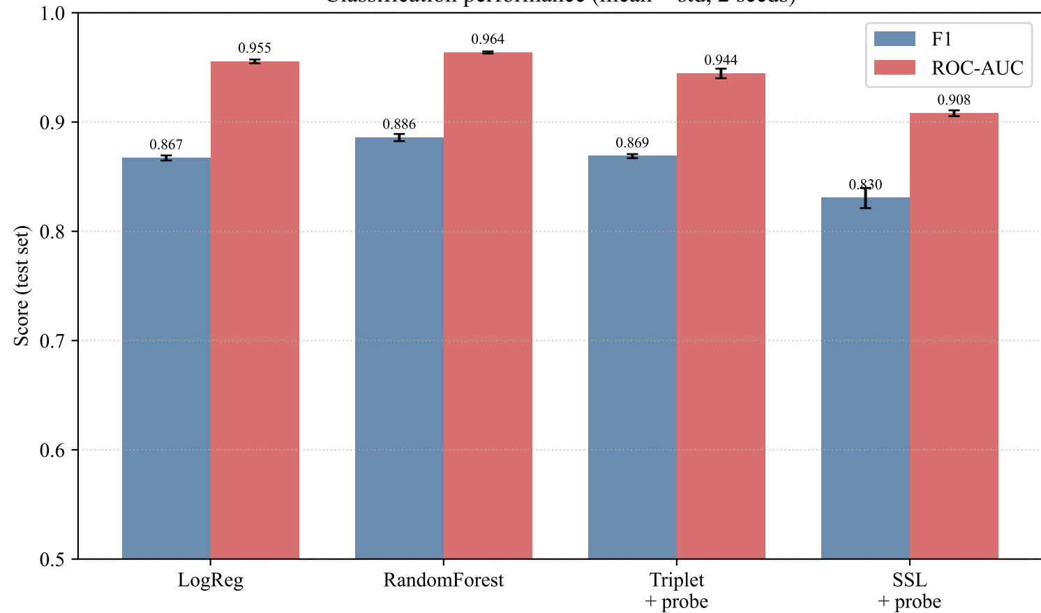
Classification performance (mean \pm std, 2 seeds)
