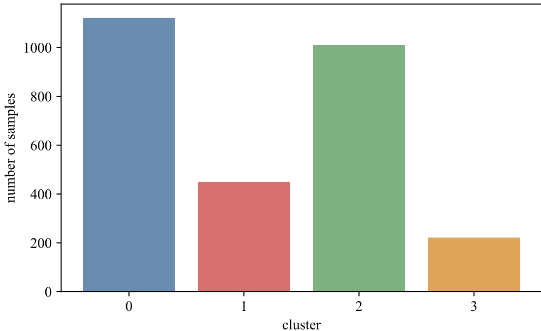
CC cluster sizes (entropy=1.228) — no collapse
