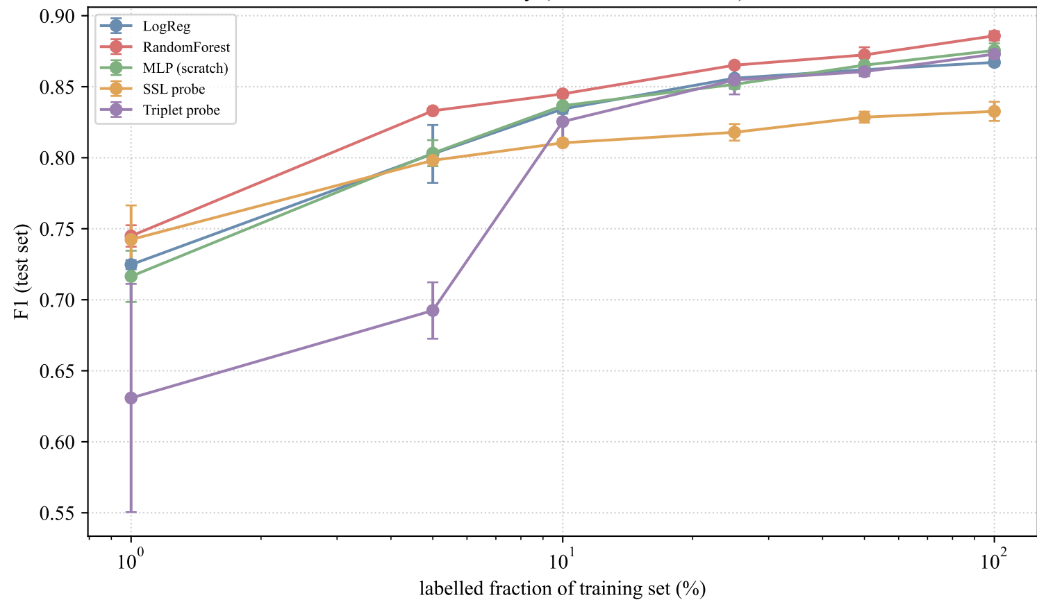
Label efficiency (mean \pm std, 2 seeds)
